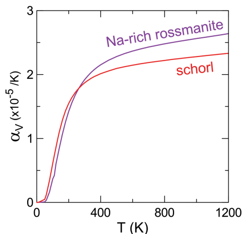
FIGURE 3. Thermal expansion coefficient vs. temperature in Na-rich rossmanite and schorl. The coefficient was calculated from the fit reported in Table 3.
