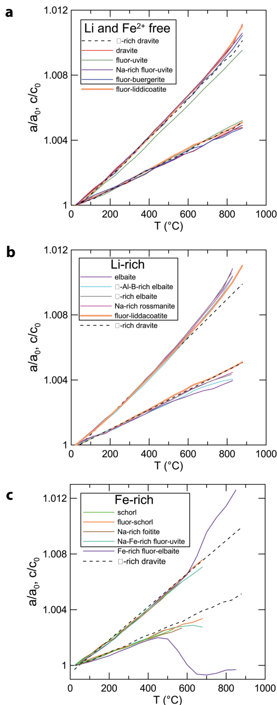
FIGURE 4. Plots of high-temperature divided by room-temperature unit-cell parameters for present samples. Lines connect experimental measurements (symbols omitted for clarity). (a) Thermal expansion of Li- and \text{Fe}^{2+} -free samples (fluor-liddicoatite added in bold for reference). (b) Thermal expansion of Li-rich tourmalines (data for \square -rich dravite added for reference, fluor-liddicoatite in bold). (c) Thermal expansion of the \text{Fe}^{2+} -rich tourmalines compared with that for dravite. Thermal behavior of \text{Fe}^{2+} -rich fluor-elbaite from Celata et al. (2021) is shown for comparison.
