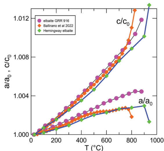
FIGURE 2. Thermal expansion of Na-rich rossmanite (formerly elbaite) GRR 916b compared with the high- T elbaite data of Ballirano et al. (2022) and Hemingway et al. (1996).
