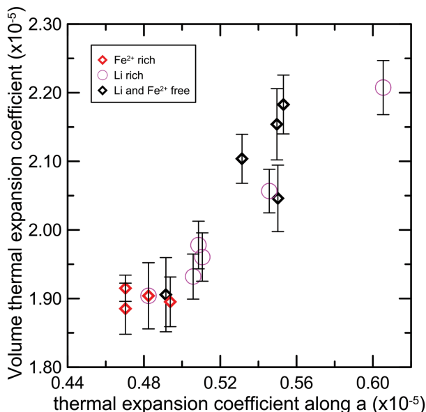
FIGURE 8. Volume thermal expansion coefficient vs. axial expansion along a ; data are from the FEI model at 298 K.
