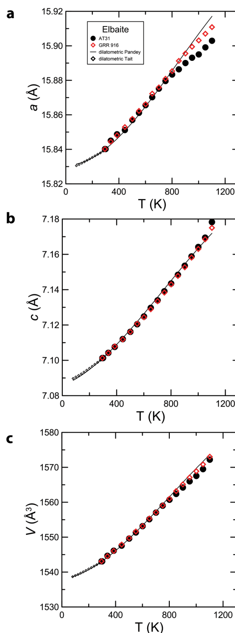
FIGURE 5. Elbaite thermal expansion: Dilatometric data were calibrated against room-temperature value of elbaite FHAT31. The data from elbaite were scaled to overlap with those for Na-rich rossmanite (GRR 916). The line is not a fit, but rather the thermal expansion from Pandey and Schreuer (2012), sample T003.
