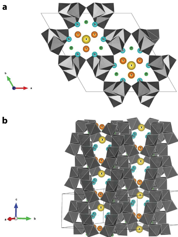
FIGURE 1. Crystal structure of tourmaline: (a) along the b axis and (b) parallel to the c axis.
