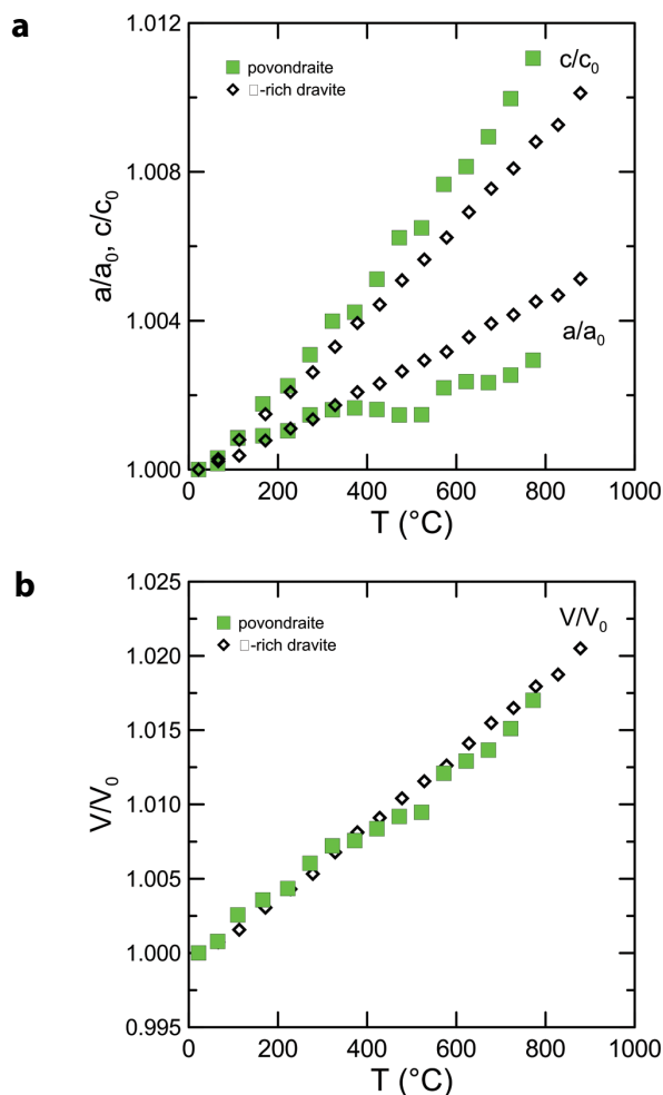
FIGURE 6. Povondraite unit cells compared with those for □-rich dravite NMNH 78719-1.
