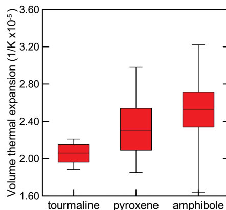
FIGURE 9. Thermal expansion variability in mineral supergroups: pyroxene and amphibole data are from Hovis et al. (2021) and Tribaudino et al. (2022), respectively, with tourmaline data from the present work. The box represents the upper and lower 25 and 75% of the data, whereas the line in between is the median; whiskers represent the minimum and maximum values.
