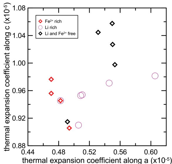
FIGURE 7. Thermal expansion along the a and c crystallographic axes. Thermal expansion according to the Fei model, fit over the range reported in Table 3.
