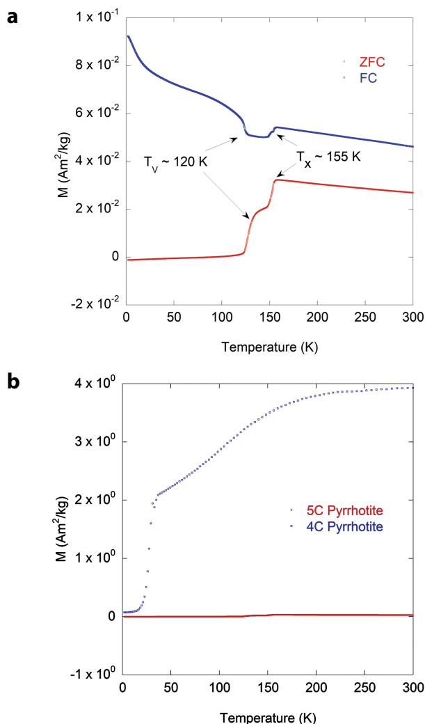
FIGURE 4. Magnetization, M , of 5C crystal. (a) ZFC and FC data, measured in a field of 10 mT ( H//a ). The anomaly at \sim 120 K is due to the presence of a small amount of magnetite (labeled as T_V for the Verwey transition) as impurity phase. The previously unknown transition is labeled as T_X . (b) Comparison with ZFC data for 4C and 5C crystals ( H//a ), showing a difference in magnetization of a factor of \sim 100 . (Color online.)
