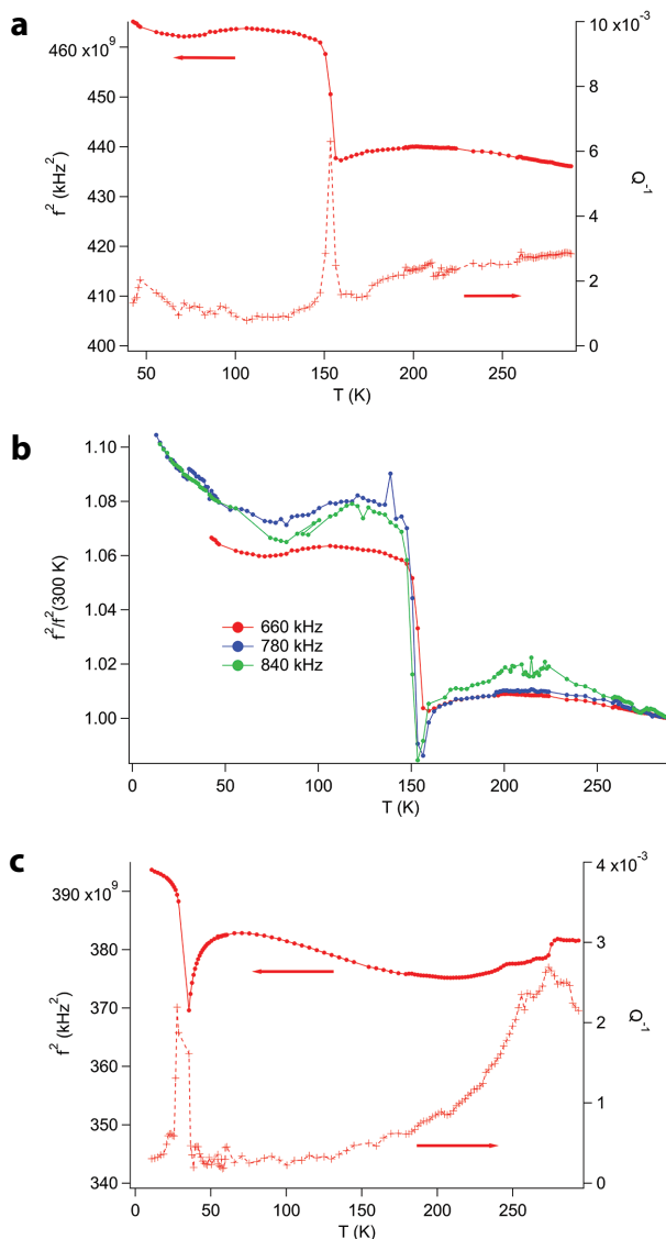
FIGURE 7. (a) Temperature dependence of f^2 and Q^{-1} for the single crystal of 5C pyrrhotite from fitting of the resonance peak near 650 kHz and (b) f^2 for three resonance peaks at 660, 780, and 840 kHz normalized to the value at room temperature. (c) Temperature dependence of f^2 and Q^{-1} for a single resonance with frequency near 620 kHz from a 4C pyrrhotite crystal cut from the same original sample as was used to produce the 5C crystal. The Besnus transition is marked by a minimum of f^2 at ~36 K. Crosses = Q^{-1} , right axis; filled circles = f^2 , left axis. (Color online.)
