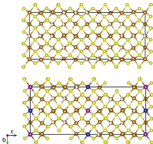
FIGURE 2. Structural model of pyrrhotite 5C viewed along [100] from this work (top) and from de Villiers et al. (2009) (bottom). Color code: yellow = S; brown = Fe (partial occupancy is shown by half-gray half-brown); pink = partially Ni replaced Fe site (de Villiers et al. 2009); blue = vacant metal site from de Villiers et al. (2009) (see main text for details). (Color online.)
