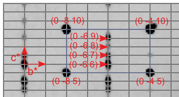
FIGURE 1. Part of the (0kl) precession image of the room-temperature single-crystal X-ray diffraction pattern, showing the fivefold superlattice reflections of the 5C structure. The data has been reduced using the cell from the Cmce structure and the peaks are labeled with the (hkl) of the Cmce structure. The direction of b^* and c^* are given in red on the left. The unit cell of the Cmce structure is shown by the gray grid. The projection of the hexagonal parent cell onto the Cmce (0kl) plane is shown in blue. The fivefold modulation in the l direction can be seen and the peaks characteristic of this are labeled with their (hkl) values. (Color online.)
