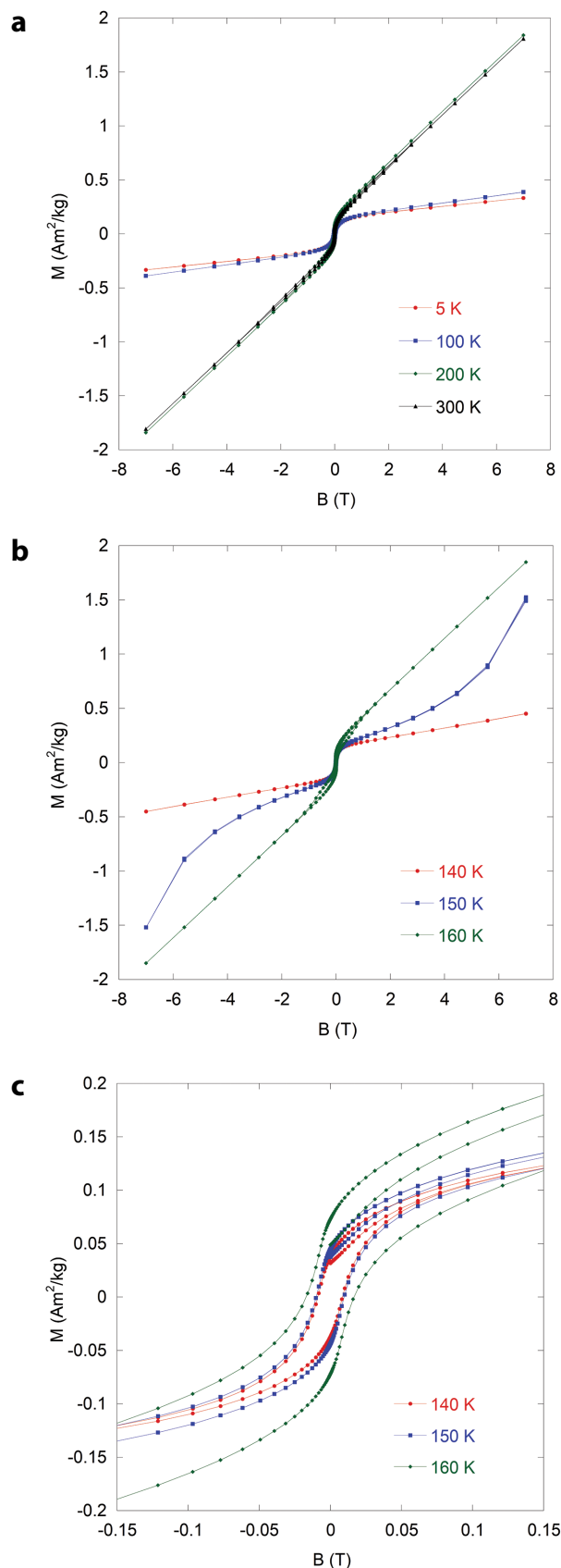
FIGURE 5. (a) Field and temperature dependence of the magnetization of the 5C sample. The field was applied parallel to the [100] direction of the parent NiAs structure unit cell ( H//a ). The structure at 200 and 300 K has marked differences in magnetic anisotropy from the structure at 5 and 100 K. Neither show any indication of saturation at high fields. (b) Field and temperature dependence of magnetization of the 5C structure close to the magnetic transition at \sim 155 K ( H//a ). (c) Close in view of the low field region from b, showing slight opening of the loops that is attributed to the presence of a small amount of magnetite. (Color online.)
