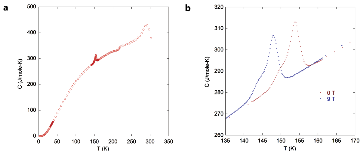
FIGURE 3. (a) Heat capacity of 5C crystal measured between 2 and 300 K in zero field, showing the magnetic transition near 155 K. Anomalies at ~215 and ~280 K are artifacts. (b) Higher resolution view of the peak at 154 K in zero field, which shifts to 148 K when measured in a 9 T field ( H//a ). (Color online.)
