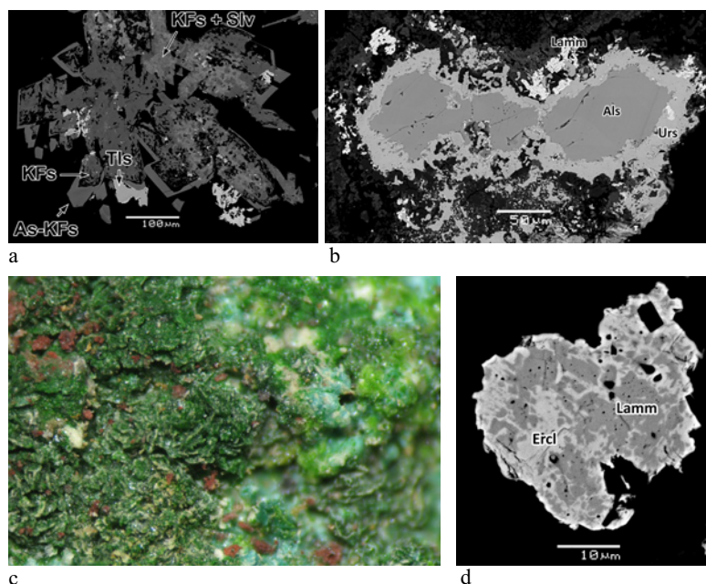
Fig. 8. Crystallization sequence of different arsenates and As-bearing potassic feldspar: (a) As-rich (16 wt% \text{As}_2\text{O}_5 ) potassic feldspar (As-KFs) overgrowing As-poor (<2 wt% \text{As}_2\text{O}_5 ) potassic feldspar (KFs), with tilasite (Tls) and sylvite (Slv); (b) alarsite (Als) surrounded by urusovite (Urs) replacement rim and overgrown by lammerite (Lamm); (c) deep-green ericlavmanite replaces urusovite crystal crust (pale blue urusovite relics and light green kozyrevskite occur in the right part of the photograph); (d) ericlavmanite (Ercl) overgrows lammerite. Arsenatnaya fumarole. (c) FOV width: 5.8 mm; (a, b and d) SEM (BSE) image.
