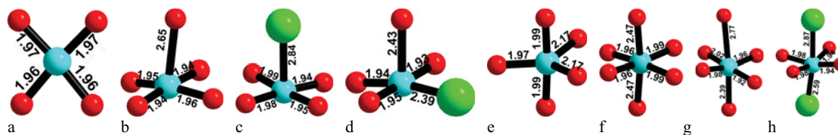
Fig. 9. Diversity of \text{Cu}^{2+} -centred coordination polyhedra in oxyarsenates from Tolbachik fumaroles: almost planar square in dmsokolovite (a); square pyramids in ericlxmanite (b), axelite (c), and coparsite (d); trigonal bipyramid in kozyrevskite (e); distorted octahedra in shchurovskyite (f), edtolite (g), and coparsite (h). Bond lengths (in Å) are marked. Blue circles are Cu, red circles are O and green circles are Cl atoms; d, h – drawn after Starova et al. (1998), others – our data.
