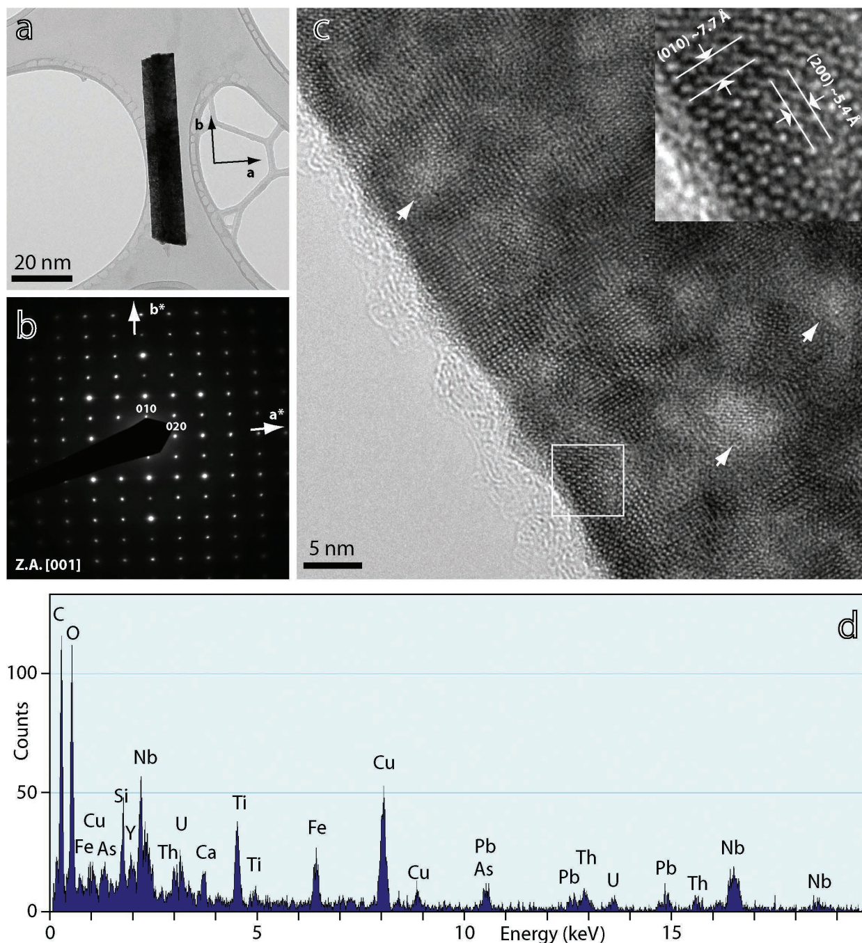
FIGURE 6. (a) BF-TEM image of an arborescent crystal picked up from the miarolitic cavity and put on a carbon coated Cu-grid and (b) related SAED taken with the incident beam parallel to [001]. This pattern is consistent, within the experimental error and net of dynamical effects— 0kl for k = 2n only—with aeschynite ( Pnma , a \sim 10.80 , b \sim 7.68 , c \sim 5.10 Å, Capitani et al. 2016). (c) HR-TEM image showing mottled contrast typical of metamict minerals, with brighter areas lacking of long-range order (arrows). The main lattice planes within a crystalline area (square) are showed (inset). (d) Representative EDS spectrum (Cu peaks are from the grid). (Color online.)
