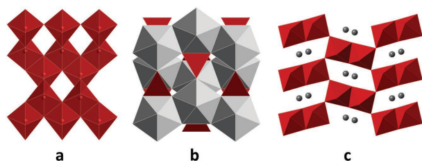
FIGURE 1. (a) \text{TiO}_6 polyhedra arrangement in the anatase structure (Horn et al. 1972) as seen down [100] ( c vertical). (b) \text{SiO}_4 and \text{ZrO}_8 polyhedra arrangement in the structure of zircon (Robinson et al. 1971) as seen down [100] ( c vertical). (c) A-site cations (gray circles) and B-site octahedra (red) arrangement in the structure of aeschynite (this study) as seen down [010] ( c vertical). These three structures are unrelated to each other, i.e., they do not share any common feature(s) such as oxygen packing or polyhedral arrangement, consistently with the lack of crystallographic orientational relationship. (Color online.)
