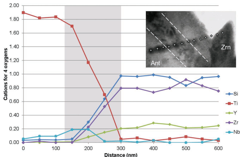
FIGURE 5. Compositional profile across the anatase/zircon interface for a distance of about 600 nm. The shadowed region in the plot corresponds to the band showing strain contrast and outlined by dashed lines in the inset. The inset also shows the trace of the compositional profile as resulting from the contamination stains formed at beam positions during spot analysis collection, which were taken at intervals of ~50 nm (crosses). Note the Nb maximum at the anatase/zircon interface. (Color online.)
