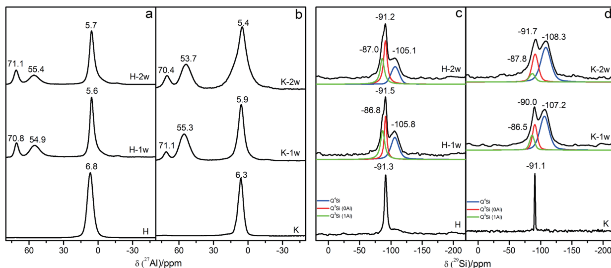
FIGURE 7. ^{27}\text{Al} (a and b) and ^{29}\text{Si} (c and d) MAS NMR spectra of halloysite, kaolinite, and their hydrothermal products. (a and c) Halloysite (H) and the products after one week (H-1w) and two weeks (H-2w) of hydrothermal treatment. (b and d) Kaolinite (K) and the products after one week (K-1w) and two weeks (K-2w) of hydrothermal treatment.
