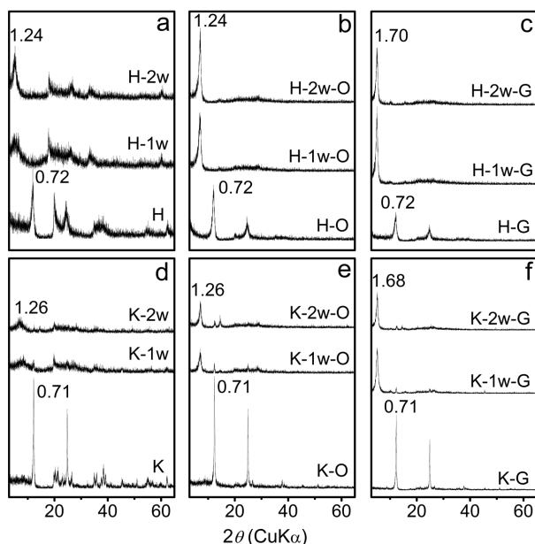
FIGURE 1. XRD patterns of halloysite, kaolinite, and their hydrothermal products with \text{Na}_2\text{SiO}_3 \cdot 9\text{H}_2\text{O} . (a) Randomly oriented halloysite (H) and its hydrothermal products (H-1w and H-2w). (b) Oriented halloysite (H-O) and its hydrothermal products (H-1w-O and H-2w-O). (c) Glycolated halloysite (H-G) and its hydrothermal products (H-1w-G and H-2w-G). (d–f) Randomly oriented, oriented, and glycolated samples of kaolinite (K) and its hydrothermal products. (O = oriented sample, G = glycolated sample.)
