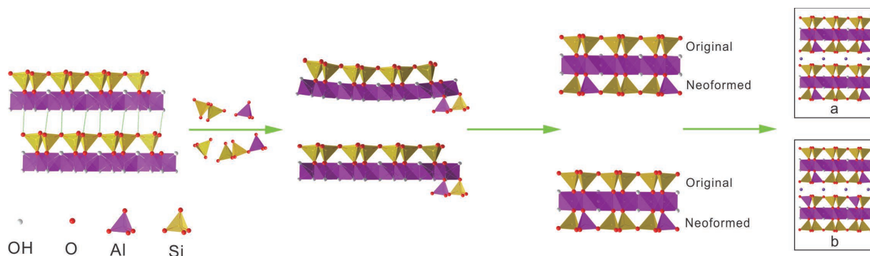
FIGURE 8. Schematic representation of the transformation from 1:1 type clay minerals to 2:1 ones. (a) The newly formed tetrahedral sheet is attached to the pre-existing 1:1 unit from the same direction. (b) The two newly formed tetrahedral sheets are attached from two opposite direction, forming a symmetry across the interlayer, which is a typical mixed layer structure with “polar layers.”
