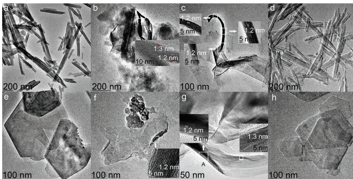
FIGURE 3. HRTEM images of halloysite, kaolinite, and their hydrothermally treated products. (a) The original halloysite. (b and c) Hydrothermally treated products of halloysite with \text{Na}_2\text{SiO}_3 \cdot 9\text{H}_2\text{O} after one and two weeks. (d) Halloysite after two weeks' dissolution experiment without \text{Na}_2\text{SiO}_3 \cdot 9\text{H}_2\text{O} (H-D-2w). (e) The original kaolinite. (f) Hydrothermally treated product of kaolinite with \text{Na}_2\text{SiO}_3 \cdot 9\text{H}_2\text{O} after one week. The parts marked with square became curved, which are composed of beidellite layers. (g) Hydrothermally treated product of kaolinite with \text{Na}_2\text{SiO}_3 \cdot 9\text{H}_2\text{O} after two weeks, beidellite layers with a thickness of 1.2–1.4 nm were extensively formed accompanied with exfoliation. (h) Kaolinite after two weeks' dissolution experiment without \text{Na}_2\text{SiO}_3 \cdot 9\text{H}_2\text{O} (K-D-2w).
