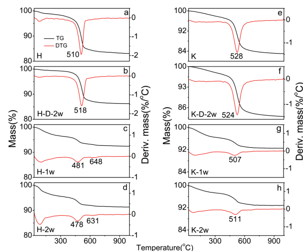
FIGURE 5. TG and DTG curves of halloysite, kaolinite, and their hydrothermally treated products. (a, c, and d) Halloysite (H) and its hydrothermal products with Na 2 SiO 3 ·9H 2 O after one week (H-1w) and two weeks (H-2w). (b) Halloysite after two weeks' dissolution experiment without Na 2 SiO 3 ·9H 2 O (H-D-2w). (e, g, and h) Kaolinite (K) and its hydrothermal products with Na 2 SiO 3 ·9H 2 O after one week (K-1w) and two weeks (K-2w). (f) Kaolinite after two weeks' dissolution experiment without Na 2 SiO 3 ·9H 2 O (K-D-2w).
