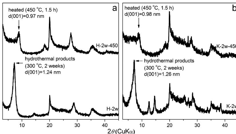
FIGURE 2. XRD patterns of the hydrothermal products of halloysite (a) and kaolinite (b) and the corresponding samples heated at 450 °C for 1.5 h.
