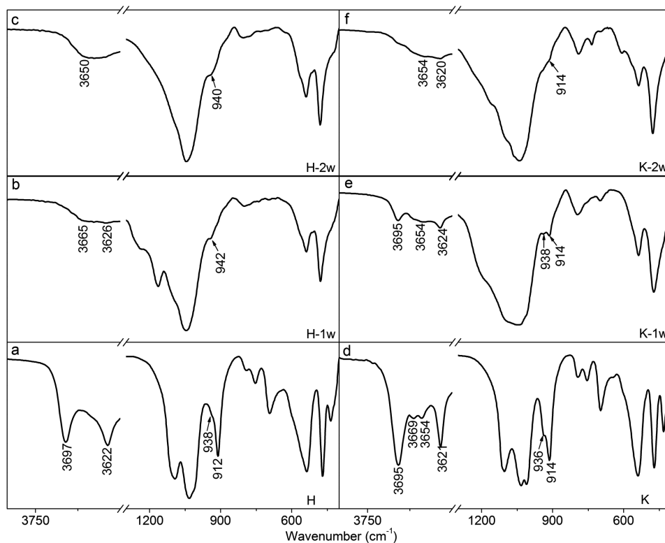
FIGURE 6. FTIR spectra of halloysite, kaolinite, and their hydrothermal products. (a–c) Halloysite (H), and its products after one week (H-1w) and two weeks (H-2w) of hydrothermal treatment. (d–f) Kaolinite (K), and its products after one week (K-1w) and two weeks (K-2w) of hydrothermal treatment.
