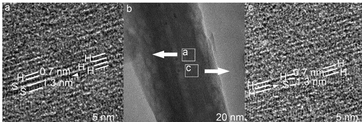
FIGURE 4. HRTEM images of the products of halloysite after 3 days of hydrothermal treatment. H = halloysite layer (0.7 nm thick); S = smectite layer (1.3 nm thick). The lateral transition H → S is indicated by arrows.
