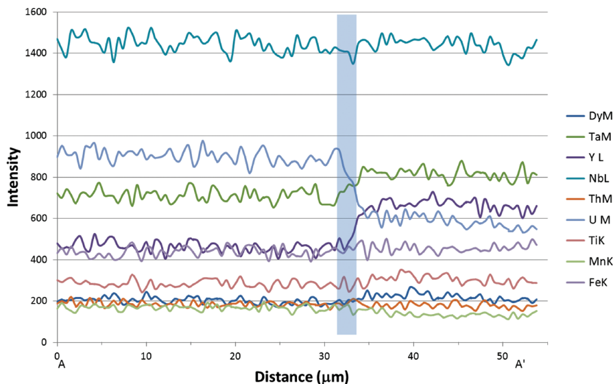
FIGURE 2. Representative compositional line scan across the two domains of the U-bearing phase (see Fig. 1b for locating the line scan). The line scan is composed of 103 points equally spaced within \sim 54 \mu\text{m} , each point counted for 10 s. The gray band represents the interface between the brighter (left) and the darker domain (right). (Color online.)
