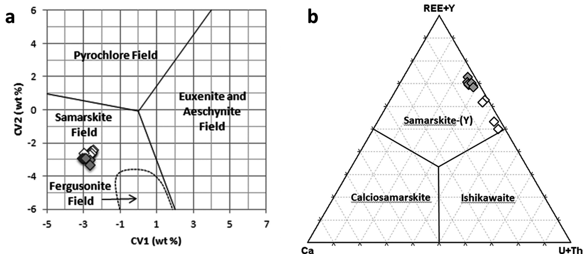
FIGURE 3. (a) Plot of the WDS microprobe compositions on the canonical variable diagram of Ercit (2005). CV1 = 0.106 \text{ Ca} - 0.077 (\text{Fe}^{2+} + \text{Fe}^{3+} + \text{Mn}) + 0.220 \text{ Y} + 0.280 (\text{Nd} + \text{Sm}) + 0.137 (\text{Gd} + \text{Dy} + \text{Yb}) + 0.100 \text{ U} + 0.304 \text{ Ti} + 0.097 \text{ Nb} + 0.109 (\text{Ta} + \text{W}) - 12.81 (\text{oxide wt\%}) ; CV2 = -0.113 \text{ Ca} - 0.371 (\text{Fe}^{2+} + \text{Fe}^{3+} + \text{Mn}) - 0.395 \text{ Y} - 0.280 (\text{Nd} + \text{Sm}) - 0.265 (\text{Gd} + \text{Dy} + \text{Yb}) - 0.182 \text{ U} - 0.085 \text{ Ti} - 0.166 \text{ Nb} - 0.146 (\text{Ta} + \text{W}) + 17.29 (\text{oxide wt\%}) . Dark diamonds = point analyses on BSE darker regions; white diamonds = point analyses on BSE brighter regions. (b) Ternary diagrams for the samarskite group minerals. From a compositional point of view, the U-bearing phases detected in the Codera dike samples can be classified as samarskite-(Y).
