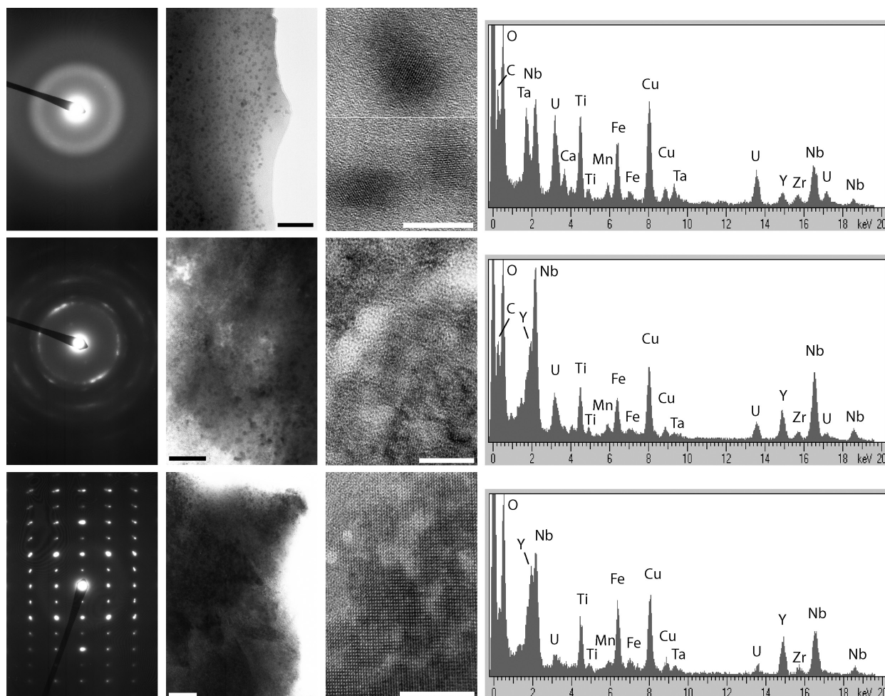
FIGURE 4. TEM images and EDS spectra at different regions of the metamict U-bearing phase detected in the Codera dike sample. Columns are organized as to show from left to right selected area diffraction patterns, bright-field images, high-resolutions images, and compositional spectra. The degree of radiation damage decreases from the top to the bottom row, corresponding to a decrease in radiogenic uranium content. Scale bar 100 nm in BF images and 10 nm in HR images.
