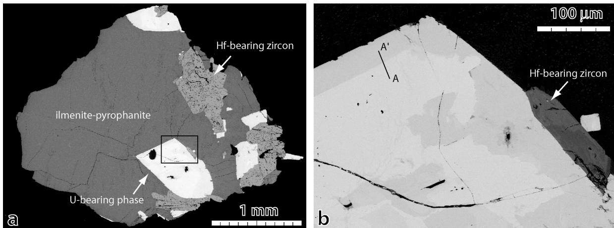
FIGURE 1. SEM-BSE images of a polished section of sample 2 (sample 1 shows analogous microstructure with similar compositions). (a) Low-magnification image showing the sample embedded in epoxy (peripheral black contrast). At least three different phases can be recognized on the basis of BSE contrast: ilmenite-pyrophanite, occupying the widest, dark gray area; Hf-bearing zircon, with intermediate gray contrast; and an U-bearing phase, with the brightest contrast. (b) High-magnification image of the area enclosed within the black rectangle in a where the zoning affecting the U-bearing phase can be appreciated. A-A' trace of the line scan (see Fig. 2).
