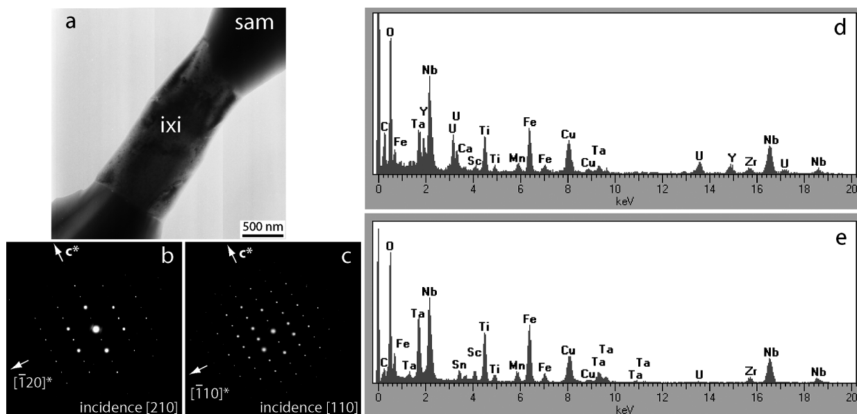
FIGURE 9. (a) BF image showing and ixiolite crystal (ixi) making a bridge between two amorphous region of samarskite-(Y) (sam). (b and c) SAED patterns recorded in ixiolite along two different directions obtained rotating the crystal around c^* . (d and e) EDS spectra taken in the amorphous region and in the crystalline ixiolite, respectively. Note the absence of U in the latter (N.B.: the Cu peaks come from the TEM supporting grid).
