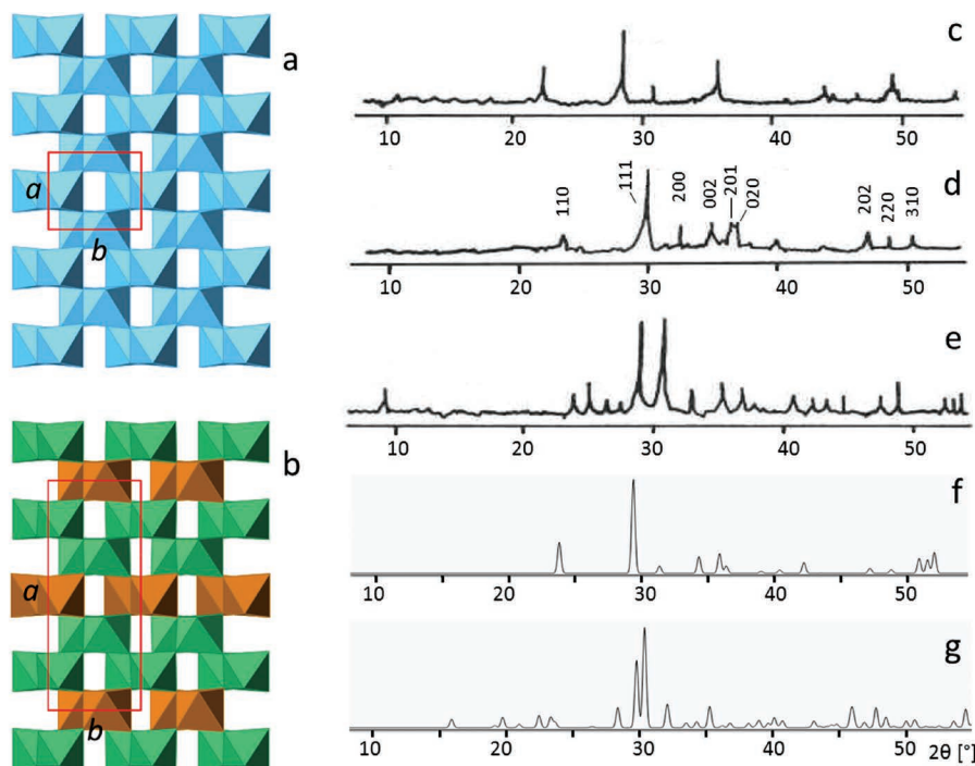
FIGURE 8. Structure of ixiolite (a) and columbite (b) showing the stacking of the octahedral cations (shadowed) as seen along [001] (different colors means different cation occupancies). Note how the ordering of octahedral cations in columbite leads to the tripling of the a parameter, making the latter a superstructure with ixiolite subcell. Powder X-ray diffractograms of samarskite-(Y) (Sugitani et al. 1984): (c) sample annealed at 580 °C in air for 12 h (upon these conditions a different phase forms); (d) annealed at 550 °C for 16 h in H 2 (these conditions lead to the low-temperature ixiolite-like structure); (e) annealed at 950 °C for 15 h in H 2 (these conditions lead to the high-temperature wolframite-like structure). Calculated powder diffractograms: (f) ixiolite with cell parameters and composition of Sugitani et al. (1984); (g) aeschynite-(Y) with structure and composition obtained in this study. (Color online.)
