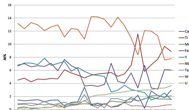
FIGURE 5. Plot of the TEM-EDS chemical analyses in several areas of the U-bearing phase ordered for increasing U-content. A clear correlation among Ti, U, Ca, Ta, and Mn is observable, as well as an anti-correlation of these elements with Nb and Y. Conversely, iron does not show any clear correlation. (Color online.)
