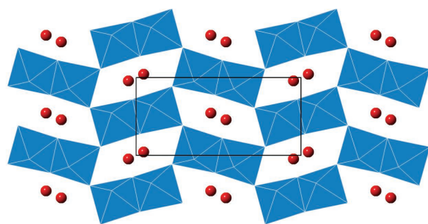
FIGURE 7. Structural sketch down the b direction of the niobiaeschnynite-(Y) as solved and refined from EDT data ( a horizontal; c vertical). The structure topology, beside an origin shift, is identical to the aeschnynite-(Y) refined by Bonazzi and Menchetti (1999). (Blue polyhedra = B-site; red circles = A-site). (Color online.)
