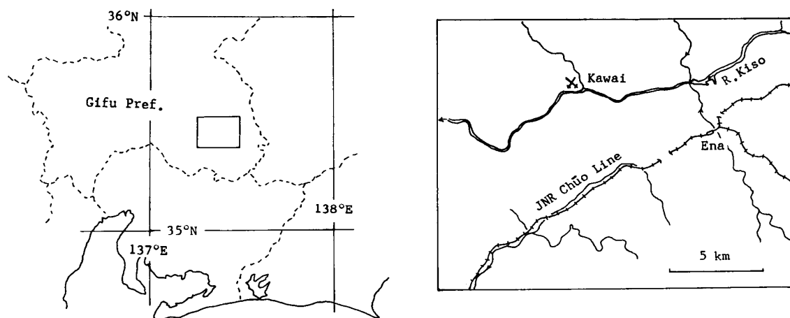
Fig. 1. Index map of the Kawai Mine (crossed hammer mark).
