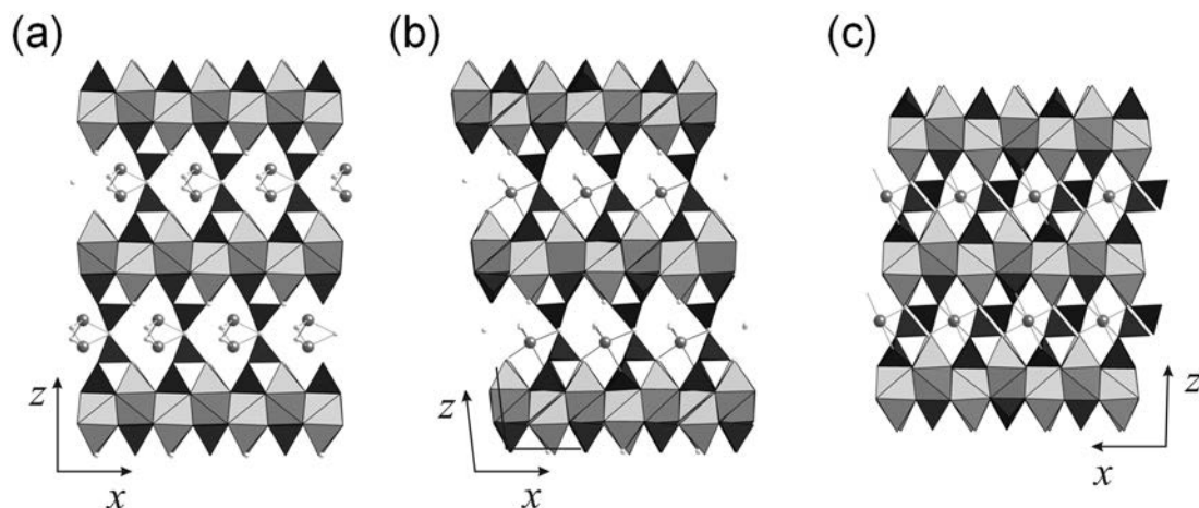
Fig. 8. The different conformation of silicate chains in tobermorite (a), clinotobermorite (b) and “tobermorite 9 Å” (c), as seen down [010]. The Si-centred tetrahedra are drawn in black, whereas the Ca-centred polyhedra are grey. Circles are (in order of decreasing size) additional Ca cations and H 2 O molecules.
