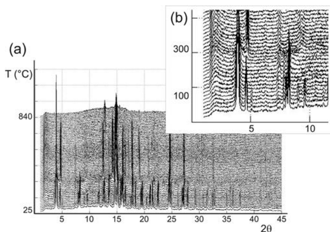
Fig. 4. X-ray powder diffraction patterns collected at the GILDA beamline upon heating. In (a) the 2\theta range 3–45° is shown, whereas the inset (b) shows the disappearance of ettringite above 100 °C and the occurrence of well crystallised “tobermorite 9 Å” at 300 °C.
