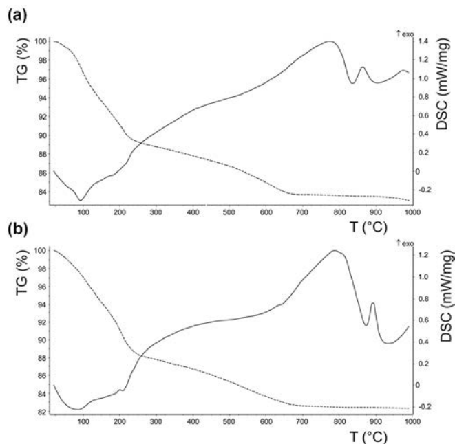
Fig. 3. TG and DSC curves (dashed and solid line, respectively) for tobermorite from Montalto di Castro (a) and Vallerano (b).
