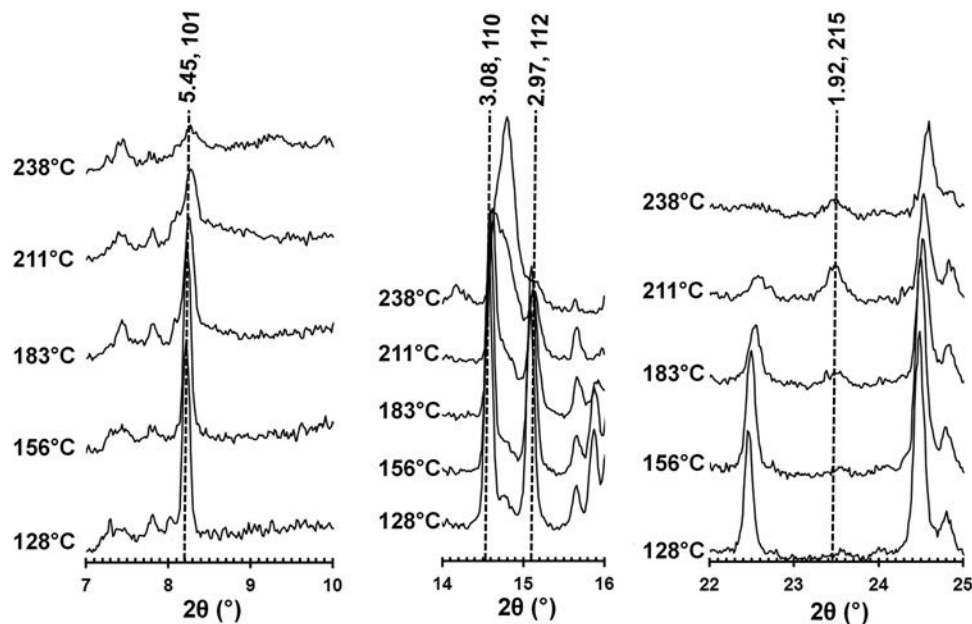
Fig. 5. The 2\theta ranges (in ^\circ ) described in the text showing the progressive disappearance of the X-ray diffraction effects related to tobermorite and the transient appearance of clinotobermorite. Diagnostic reflections are marked with their d_{hkl} spacing (in \text{\AA} ) and hkl indices.
