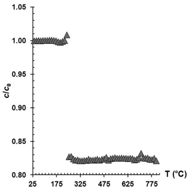
Fig. 7. The relative variation in the unit-cell parameter c (related to the basal spacing) in tobermorite and “tobermorite 9 Å” with respect to the unit-cell parameter c_0 of tobermorite at room temperature.
