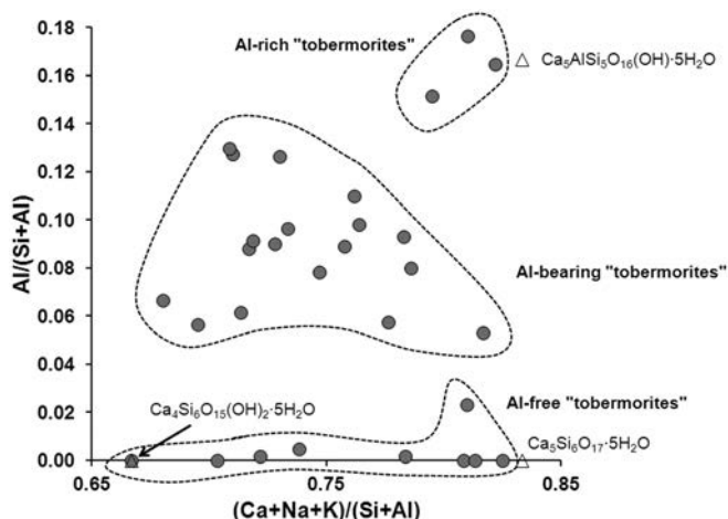
Fig. 2. Chemical variability in natural 11 Å members of the tobermorite supergroup.
