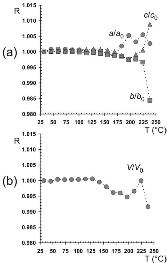
Fig. 6. Relative variations R of the unit-cell parameters (a) and unit-cell volume (b) for Al-rich tobermorite from room temperature up to its disappearance.
