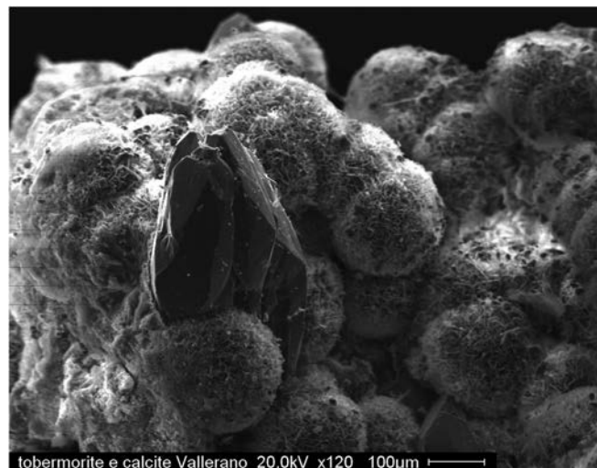
Fig. 1. Globular aggregates of thin platy crystals of tobermorite associated with calcite. Vallerano, Latium, Italy.
