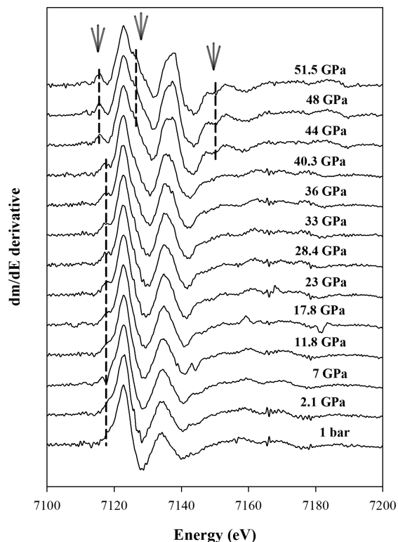
FIGURE 11. \delta\mu/\delta E derivatives of room-temperature XANES spectra of \text{FeCO}_3 at the indicated pressures. The vertical unit is arbitrary, and the derivatives are taken from the normalized spectra (Fig. 10). Gray arrows and dashed lines indicate the energies at which changes are observed at 44 GPa.
