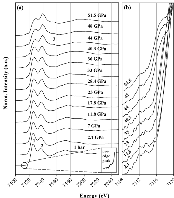
FIGURE 9. (a) Normalized XAS spectra of \text{FeCO}_3 at room temperature collected on compression at the indicated pressures. The inset at the bottom right highlights the pre-edge region of the 1 bar spectrum. (b) Close-up on the evolution of the pre-edge region with pressure. The spectra are shifted vertically for clarity.
