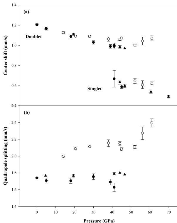
FIGURE 3. Room-temperature center shift (a) and quadrupole splitting (b) (relative to \alpha\text{-Fe} ) of \text{FeCO}_3 as a function of pressure. Solid circles = in-house single-crystal experiments; open circles = in-house powder experiment; solid triangles = SMS single-crystal experiment.
