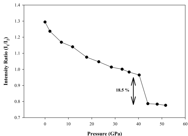
FIGURE 12. Pressure variation of the intensity ratio ( I_1/I_2 ) of the main peaks (see Fig. 9) of \text{FeCO}_3 XANES spectra. The percentage change at the transition pressure is indicated.
