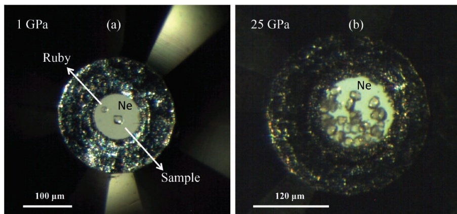
FIGURE 1. Photographs of \text{FeCO}_3 samples in DACs at the indicated pressures with (a) one single crystal and (b) multiple single crystals, each surrounded by Ne. Both loadings contain a small ruby crystal as a pressure calibrant. (Color online.)
