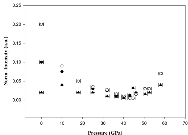
FIGURE 8. Pressure variation of Raman mode intensity normalized to the most intense mode, A_{1g} , in \text{FeCO}_3 . Solid circles = lower frequency external E_g vibration; open circles = higher frequency external E_g vibration; solid triangles = internal E_g vibration (see also Figs. 7 and 8). Note that the lowest frequency external E_g mode disappears completely above 45 GPa.
