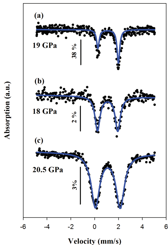
FIGURE 4. Comparison of room-temperature \text{FeCO}_3 Mössbauer spectra: (a) SMS collected on one single crystal at 19 GPa; (b) in house collected on multiple single crystals at 18 GPa; and (c) in house collected on powder at 20.5 GPa. The area asymmetry of the doublet in a is due to polarization of the synchrotron Mössbauer source. Percentage bars indicate the relative absorption. (Color online.)
