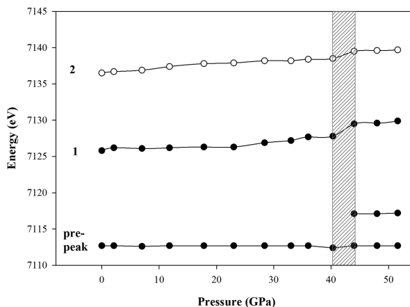
FIGURE 10. Pressure variation of maximum peak positions for \text{FeCO}_3 XANES spectra. The peaks are labeled according to Figure 9 and the gray dashed area indicates where the transition is observed in the XANES spectra.
