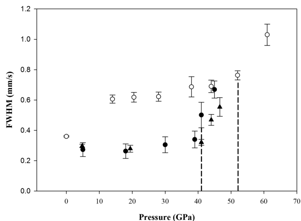
FIGURE 5. Effect of pressure on the full-width at half-maximum (FWHM) of \text{FeCO}_3 spectra. Open circles = in house powder; solid circles = in-house single crystals; solid triangles = SMS single crystal. Dashed lines indicate the pressure at which spin crossover starts for single crystal ( 41\text{ GPa} ) and powder ( 52\text{ GPa} ) measurements.
