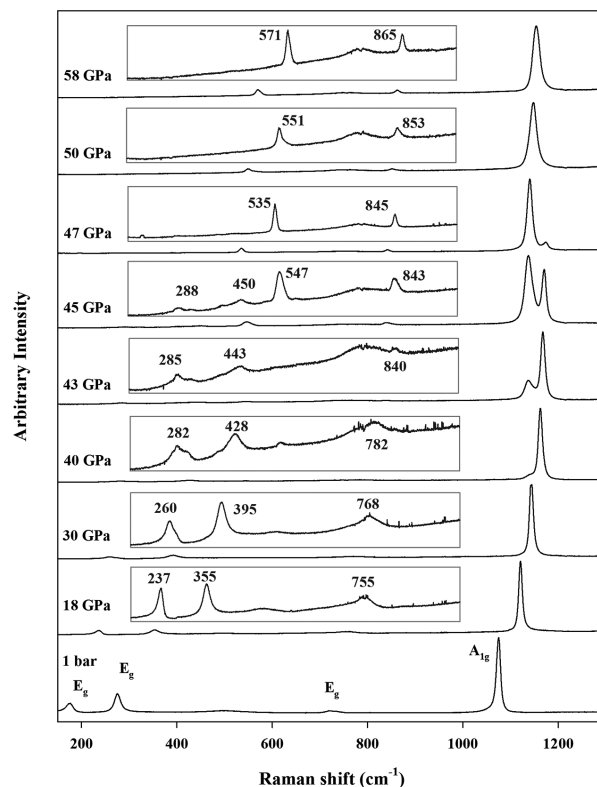
FIGURE 6. Raman spectra of \text{FeCO}_3 collected at ambient temperature and the indicated pressures. The two modes below 500\text{ cm}^{-1} are external or lattice vibrations of \text{CO}_3^{2-} relative to Fe atoms, while modes above 700\text{ cm}^{-1} are internal vibrations of \text{CO}_3^{2-} . The insets indicate the lower frequency Raman bands for the spectra on a different scale.
