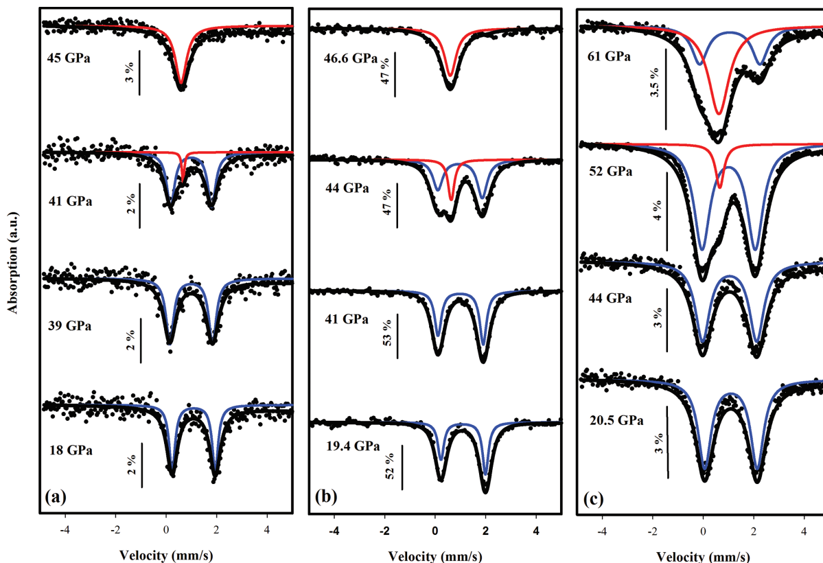
FIGURE 2. Room-temperature Mössbauer spectra of \text{FeCO}_3 (a) single crystals and (c) powder collected in house at the indicated pressures. (b) SMS spectra of one \text{FeCO}_3 single crystal collected at ESRF, Grenoble (France). Solid circles = experimental data; black lines = full transmission integral fit; blue and red lines = individual subspectra. Note that the subspectra do not add up to the total spectrum due to the properties of the full transmission integral fit. Percentage bars indicate the relative absorption. (Color online.)
