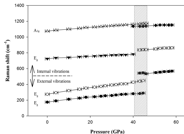
FIGURE 7. Pressure variation of the peak shift of observed Raman modes of \text{FeCO}_3 . Dashed gray area indicates the spin crossover pressure range. The frequency uncertainty is smaller than the size of the symbols.
