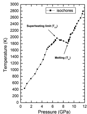
FIGURE 2. Variation of temperature vs. pressure (Z-method) showing the three parts: solid, intermediate, and liquid.
