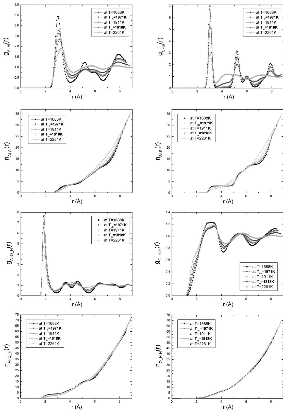
FIGURE 4. Radial distribution function g(r) showing the solid state (repeated peaks) and liquid-like state with flat curve as well the corresponding coordination numbers n(r) for various temperatures.
