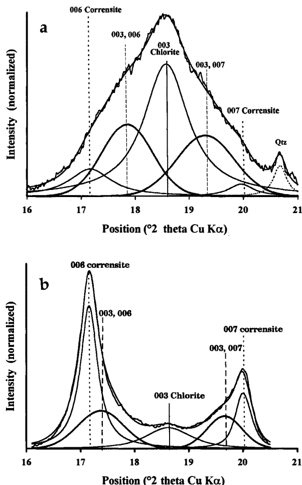
FIGURE 12. Decomposition of the peak near the chlorite 003 position of the EG-solvated samples SC1379 (a) and SC1603 (b). Dashed lines depict the 006 and 007 peaks of the corrensite diffraction pattern, and solid lines depict the position of the chlorite 003 reflection.
