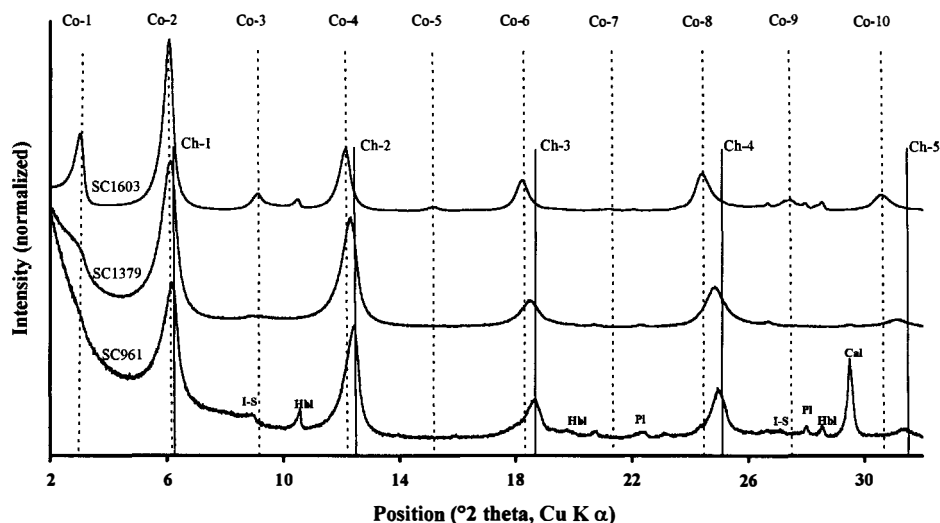
FIGURE 5. XRD patterns of air-dried correxsite (SC1603) and mixed-layer chlorite minerals with chlorite >50\% (SC1379 and SC961) that were encountered in the Sancerre-Couy deep drill hole. Dashed lines depict the 001 peaks of the correxsite diffraction pattern, and solid lines show the positions of the chlorite reflections. Hbl = hornblende, I-S = illite-smectite mixed layer, Cal = calcite, Pl = plagioclase.
