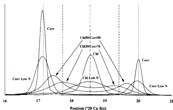
FIGURE 14. Calculated X-ray diffraction patterns of randomly interstratified ( R = 0 ) C-C mixed-layer minerals. Ethylene glycol-solvated corrensite layer: d_{001} = 31.05, ^{56}\text{Fe} = 1.0, brucitic Fe = 0.0, exchange capacity = 0.4; chlorite layer: d_{001} = 14.3, ^{56}\text{Fe} = 1.4, brucitic Fe = 0.0, brucite layer = 1.0. Coherent-scattering domain size ranges from 5 to 15 layers, except for low- N chlorite and corrensite ( 3 \leq N \leq 6 ). Dashed lines show the positions of elementary lines associated with corrensite (short dash), C-C mixed layer (long dash), and chlorite (irregular dash).
