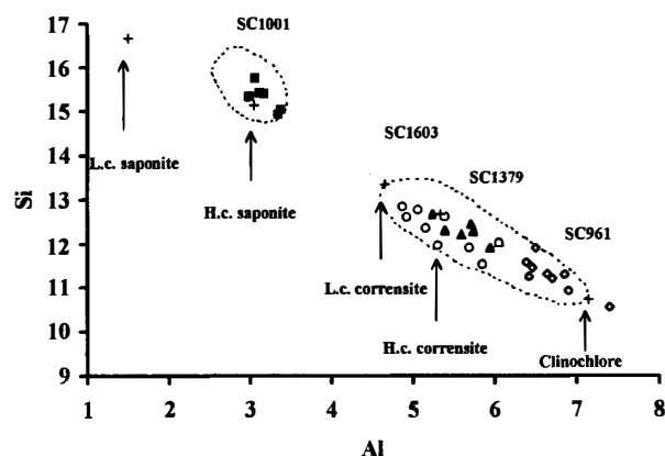
FIGURE 1. Si vs. total Al for samples SC1001, SC1603, SC1379, and SC961 on the basis of O 46 (OH) 20 . The compositions of ideal low-charge (L.c.) and high-charge (H.c.) saponite and corrensite, as well as the composition of clinocllore, are given for reference. Dashed regions correspond to EMPA data, and symbols correspond to AEM data.
