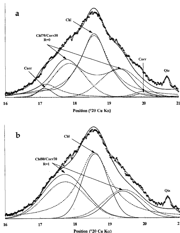
FIGURE 15. Comparison between experimental (EG-solvated sample SCI379 = plus signs) and simulated X-ray patterns in the 16–21° 2 \theta CuK \alpha range. (a) Dashed lines represent the decomposition of this band in five elementary peaks (see Fig. 12a). Solid lines represent the mixture of calculated (see Fig. 14) chlorite, corrensite, and 70:30 C-C mixed layer ( R = 0 ). A linear background was added both to the mixture of calculated patterns and to the sum of fitted elementary peaks. (b) Dashed lines represent the decomposition of this band in three elementary peaks. Solid lines represent a calculated 80:20 C-C mixed layer ( R = 1 , P_{\text{corr-chl}} = 0.65 ) and the elementary contributions to this calculated pattern as determined from decomposition. A linear background was added both to the calculated pattern and to the sum of fitted elementary peaks.
