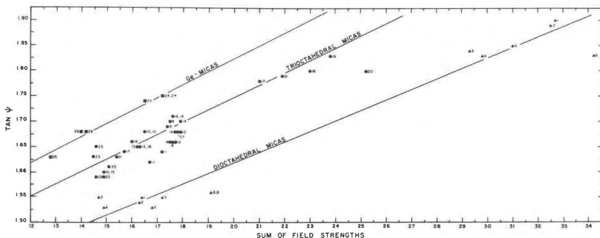
Fig. 5. Plot of \tan \psi against the sum of the field strengths of neighboring octahedra. Sheet misfit, TM, is given in listing below. Squares, circles and triangles are for germanite, trioctahedral and dioctahedral micas, respectively. (1) Rothbauer, 1971, 1.08; (2), (3) Guven, 1971, muscovite: 1.08, phengite: 1.07; (4) Zhoukhilistov et al. , 1973, 1.07; (5) Guggenheim and Bailey, 1978, 1.12; (6) this study, 1.13; (7) Joswig, 1972, 1.07; (8) Hazen and Burnham, 1973, phlogopite: 1.07; (9) Rayner, 1974, 1.07; (10) Donnay et al. , 1964, 1.07; (11) Hazen and Burnham, 1973, annite: 1.05; (12) Takeda et al. , 1975, biotite-2M 1 : 1.07; (13) Toraya et al. , 1978b, 1.05; (14) Takeda et al. , 1975, biotite-1M: 1.07; (15) Toraya et al. , 1976, 1.05; (16) McCauley et al. , 1973, 1.07; (17) Swanson and Bailey, 1981, 1.08; (18), (19) Guggenheim, 1981, lepidolite-2M 2 : 1.08, 1M: 1.08; (20) Takeda et al. , 1971, 1.07; (21) Takeda et al. , 1969, 1.07; (22) Toraya et al. , 1977, 1.05; (23) McCauley et al. , 1973, 1.07; (24) Toraya et al. , 1978c, 1.12; (25), (26) Toraya et al. , 1978a, Li-poor mica: 1.11, Li-rich mica: 1.11.
