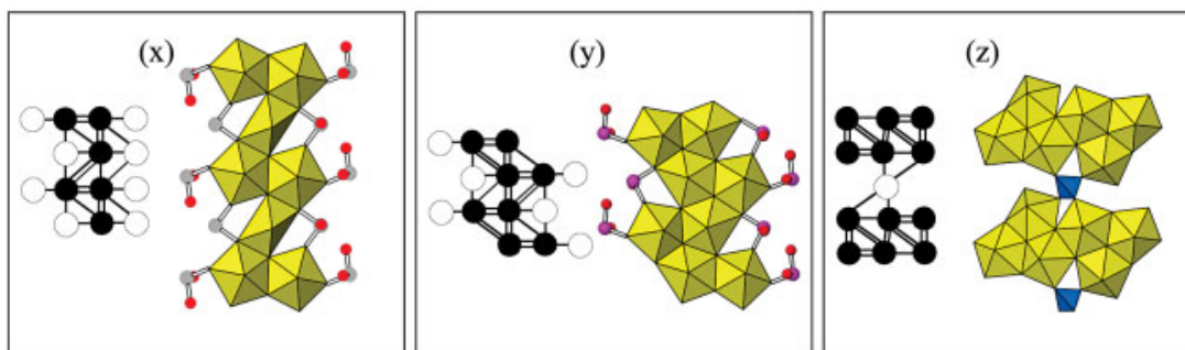
FIG. 5. Chains (and their graphical representations) of uranyl polyhedra and other polyhedra containing higher-valence cations that occur in the structures of uranyl compounds. The corresponding compounds are listed in Table 3.
