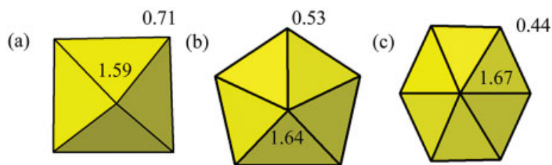
FIG. 3. Uranyl polyhedra and the corresponding average bond-valence (in valence units, vu ) incident upon each vertex owing to the U^{6+} -O bond within the polyhedron.
