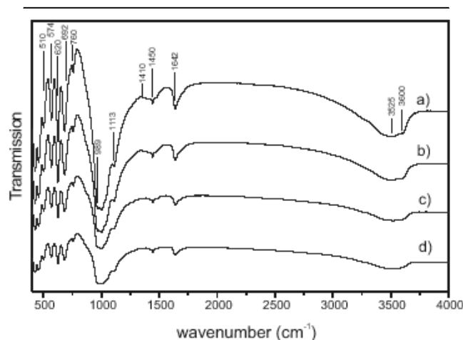
Fig. 3. IR spectra of a) sample A1, b) sample C1, c) sample O1 and d) sample O2 at 296 K.
