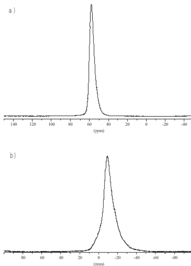
Fig. 8. ^{27}\text{Al} MAS NMR spectrum of a) sample A1, and b) ^{23}\text{Na} MAS NMR spectrum of sample C1.
