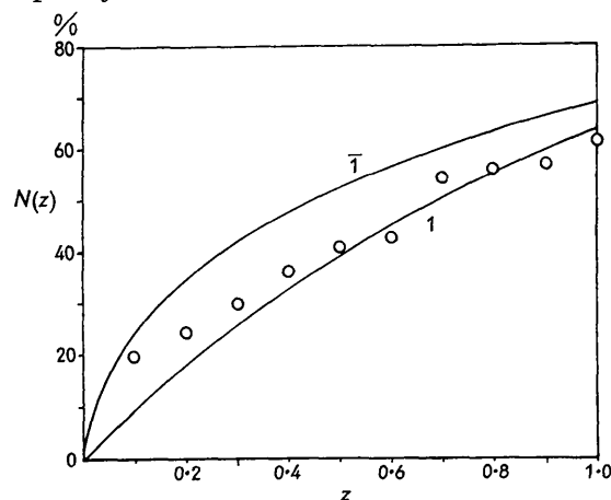
Fig. 3. N(z) test applied to the 'a'-type 0kl reflections of anorthite.
