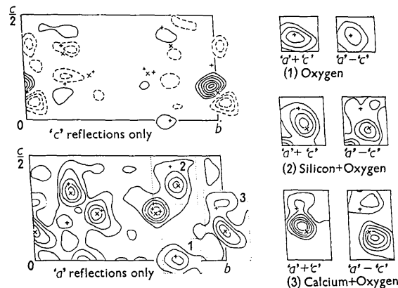
Fig. 7. Combination of 'a' and 'c' synthesis by sum and difference. Diagram shows projections on (100). Contours for 'a' at intervals of 6 e.Å -2 , zero and first contours omitted; contours for 'c' at intervals of 3 e.Å -2 , zero contour omitted. The small diagrams to the right show the effect of taking the correspondingly-numbered regions of the 'a' synthesis and adding or subtracting the electron densities in the same regions of the 'c' synthesis. Cation peaks ×, anion peaks +.
