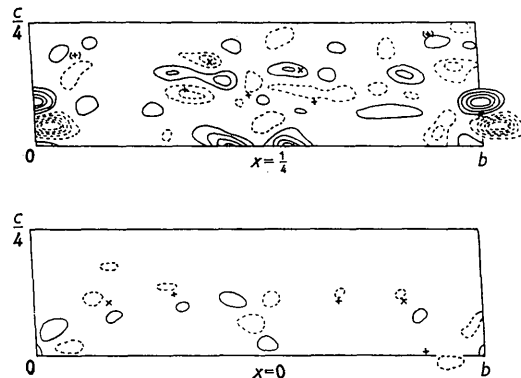
Fig. 5. 'Partial-c' synthesis, using only the strongest 'c' reflections with signs determined by Ca. Diagram shows slabs of bounded projection at x=0 and x=\frac{1}{4} . Contours at intervals of 1.5 \text{ e} \cdot \text{\AA}^{-3} ; zero contour omitted; negative contours shown dotted. Cation peaks \times , anion peaks + . The peaks near (\frac{1}{4}, \frac{1}{4}, 0) are false detail which disappears later.
