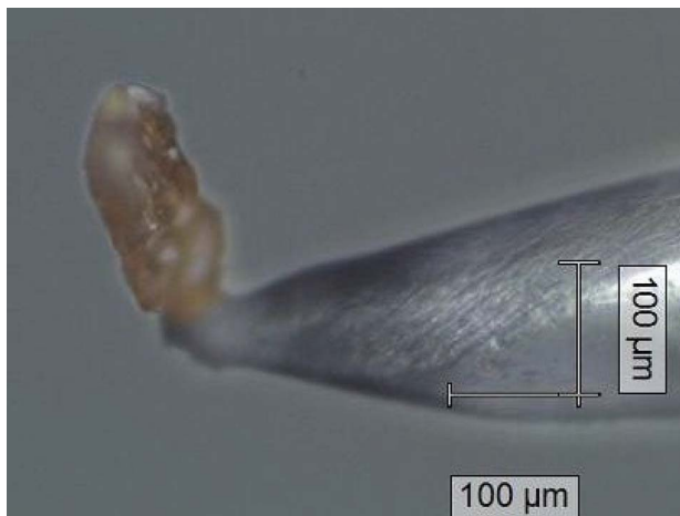
Figure 1. Pale brownish-yellow crystal of ferroinnelite ( 0.140 \times 0.070 \times 0.035 mm) on a glass fibre. This crystal was used for IR-spectroscopy at INFN-Laboratori Nazionali di Frascati (Roma), Italy.
