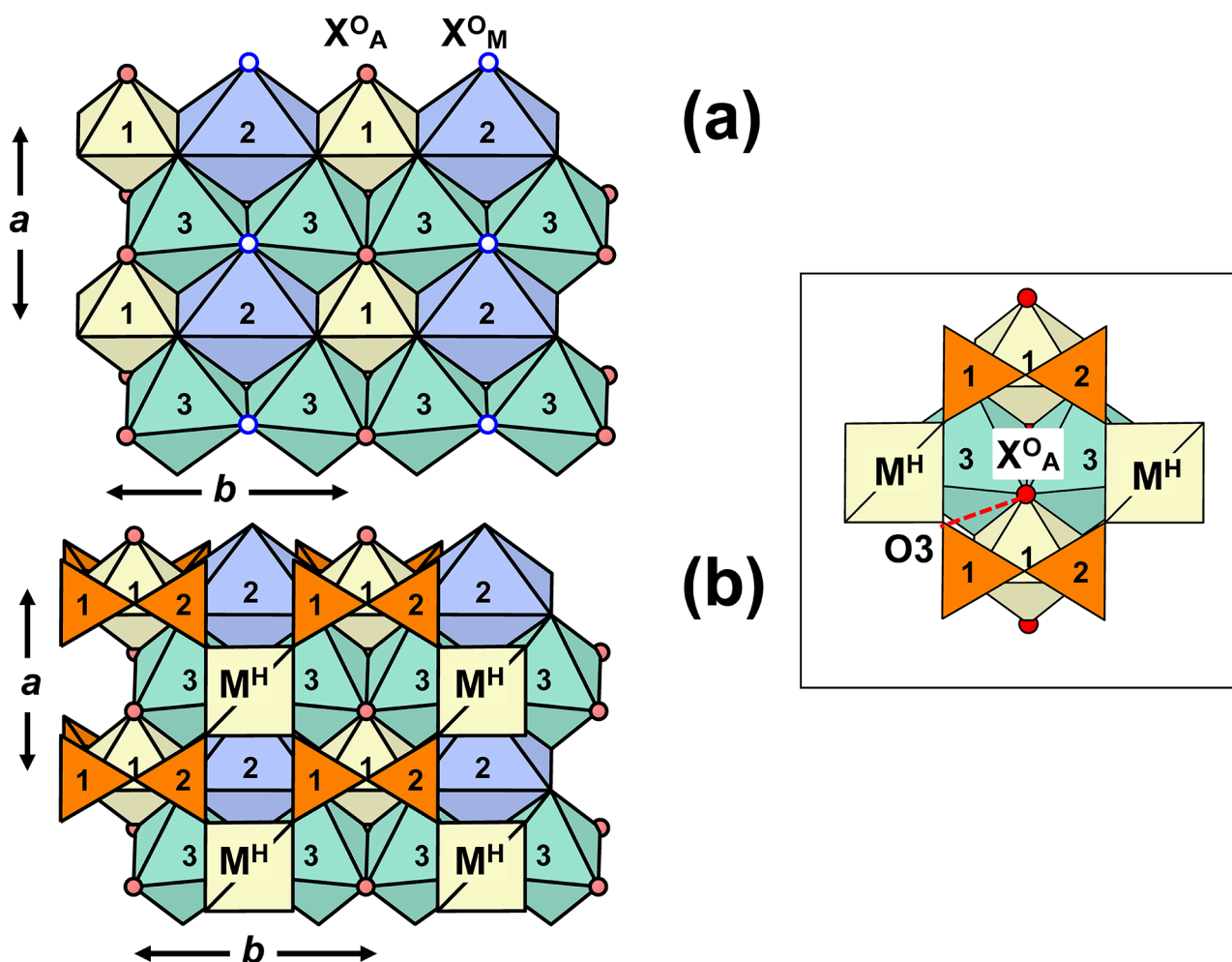
Figure 3. The TS block in the crystal structure of ferroinnelite viewed down [001]: (a) O sheet and (b) linkage of H and O sheets; \text{SiO}_4 tetrahedra are orange, \text{Ti}^{4+} -dominant polyhedra are yellow, Na octahedra and (\text{Na}, \text{Fe}^{2+}) octahedra are navy blue and bluish-green, respectively; \text{X}^{\text{O}}_{\text{M}} [O] and \text{X}^{\text{O}}_{\text{A}} [O, (OH)] anions are shown as small white circles with green rims and pink spheres. Labels 1 and 2 (on orange) correspond to \text{Si}(1,2) tetrahedra, respectively. Labels 1–3 correspond to \text{M}^{\text{O}}(1-3) octahedra in the O sheet, respectively. Inset on the right shows a possible hydrogen bond \text{X}^{\text{O}}_{\text{A}}-\text{O}3 where the \text{M}^{\text{O}}3 site is occupied by Na and the \text{X}^{\text{O}}_{\text{A}} site is occupied by an OH group shown as a small red sphere. The structure diagrams were drawn using Atoms 6.4 software (Dowty, 2016).
