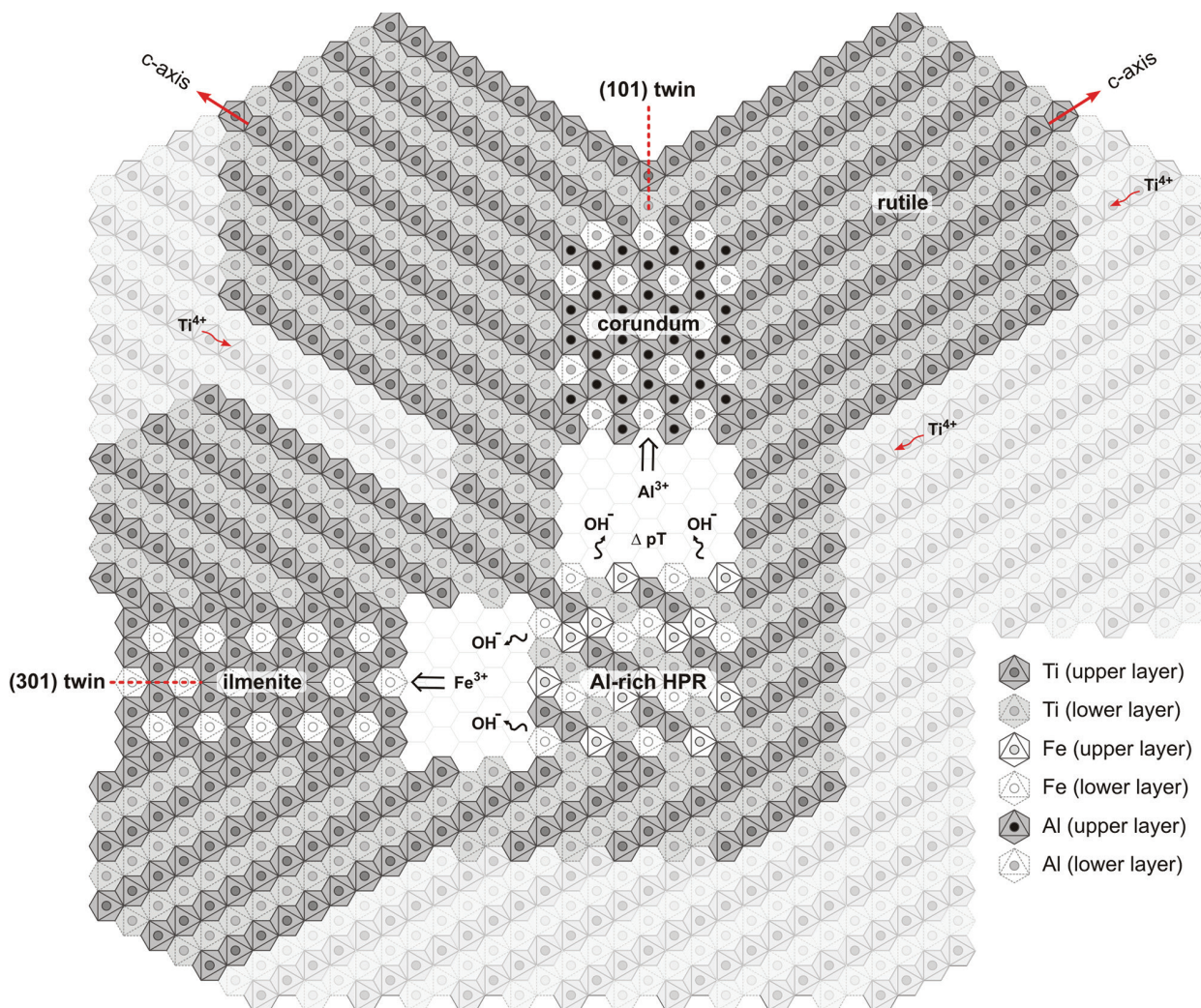
FIGURE 8. Schematic presentation of the formation of (101) and (301) rutile twins on Al-rich hydroxylan pseudorutile (HPR) precursor (Grey et al. 2010). In the beginning of the dehydration process, rutile starts to crystallize from the Al-rich HPR with a tivanite-type structure. Rutile nucleates on the surface of the precursor and progressively replaces this primary mineral. Depending on the coincidence of oppositely growing rutile domains, (101) and (301) twins can be formed. Due to tetragonal distortion of rutile, (Fe,Ti)-rich oxyhydroxide (pseudorutile) will be preferably segregated to {301} planes, whereas Al-rich oxyhydroxide (diaspore) better matches the {101} planes of rutile (see Table 1). In the final stage of dehydration the remaining oxyhydroxides are converted to oxides, ilmenite, and corundum. The resulting orientation relationship for ilmenite-rutile interface is [0001]_i \parallel [1\bar{1}00]_i \parallel [010]_R (301)_R , and that for corundum-rutile is [0001]_C \parallel [11\bar{2}0]_C \parallel [010]_R (101)_R . Note that the orientation of rutile and the precipitated corundum-type layer stays identical, only the interface is different. For simplicity, a common hexagonal oxygen framework is assumed.
