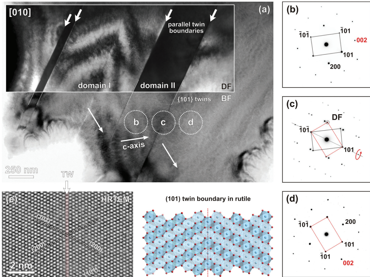
FIGURE 3. (a) Bright-field (BF) TEM image of parallel \{101\} twin boundaries in rutile viewed along [010] projection with an inset showing a dark-field (DF) image produced with a \{101\} reflection. (b–d) SAED patterns from the areas marked in a show that crystal domains across the interfaces are in twin orientation. The DF image is produced with a reflection from domain I, marked in c, and consequently domain II appears dark. (e) HRTEM image of a single (101) twin boundary (TW; highlighted red) with a simple structural model, as proposed by Takeuchi and Hashimoto (1990).
