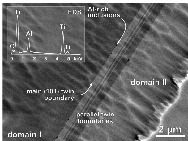
FIGURE 2. FEG-SEM/BSE image of the surface of the TEM specimen, prepared close to the [010]_R zone axis, containing (101) twin boundary at the center. The twin domains are made visible through channeling effects, where lattice planes of domain I are in better alignment with respect to the incident electron beam than those of domain II. The main (101) twin is characterized by a series of tiny black inclusions lined along the twin interface. EDS analysis revealed that these inclusions contain aluminum. Secondary (101) twins, which are visible in the right twin domain, typically contain fewer Al-rich inclusions. Waviness of the surface results from ion-milling of the specimen.
