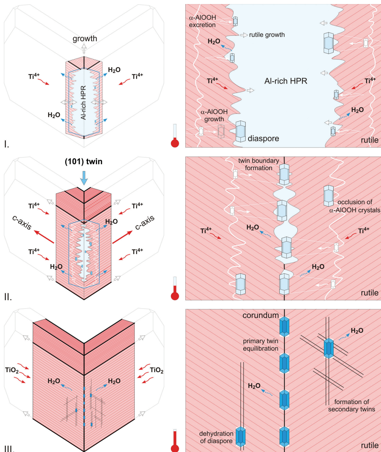
FIGURE 7. Genesis of (101) twins from Diamantina, based on nanoscale structural analysis of the specimens. Their formation involves three stages: (I) dehydration of Al-rich hydroxyl pseudorutile (HPR); (II) primary twin formation and growth; and (III) dehydration of diaspore and the formation of secondary parallel twin pairs. In the first stage, rutile starts to replace the primary (Ti, Al)-oxyhydroxide mineral through its dehydration and diffusion of \text{Ti}^{4+} ions into the hosting structure, while on the surface, rutile grows epitaxially following the structural pattern defined by the initial rutile orientation. During dehydration, Ti-dominated oxyhydroxide is converted into rutile, while Al gets excreted in form of minute diaspore nanoparticles on the crystallization front. When Al-rich domains become too large for diffusional drifting through permeable tivanite-type structure, they become occluded. In the course of replacement two rutile domains eventually meet at the center of originating oxyhydroxide, forming a twin boundary, where the majority of diaspore particles are collected. With elevated temperature, corundum is formed in place of diaspore as the final dehydration product. To compensate lattice strains after dehydration secondary twins are formed in rutile.
