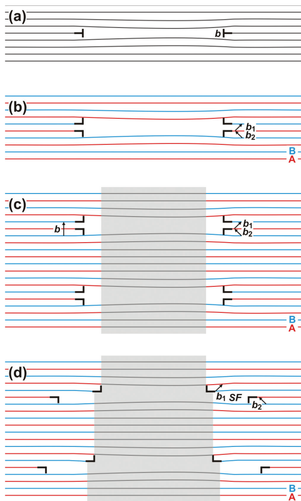
FIGURE 6. Dissociation of misfit dislocations as observed at the corundum-rutile interface. (a) A simple vacancy loop in fcc metals. (b) Due to the AB stacking of oxygen planes in rutile \mathbf{b} = [010]_R it is split into two partial dislocations \mathbf{b}_1 and \mathbf{b}_2 . (c) Simple vacancy loops in rutile with \mathbf{b} = [010]_R surrounding a corundum particle and (d) misfit dislocations \mathbf{b} = [010]_R dissociated into \mathbf{b}_1 and \mathbf{b}_2 separated by a stacking fault (SF). The \mathbf{b}_1 is usually pinned at the interface step of corundum, whereas \mathbf{b}_2 is located at the other end of the SF.
