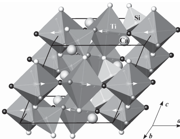
FIG. 1. Crystal structure of titanite. Lines represent the unit-cell boundaries. Arrows within \text{TiO}_6 octahedra represent off-center displacement of six-coordinated atoms from the ideal position observed in the \text{CaTiOSiO}_4 , which disappears in the Na–Nb- and Nb–Al-doped synthetic titanite. The O(1), O(2) and O(3) atoms are shown as small black, light grey and grey spheres, respectively.
