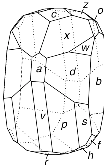
FIG. 2. Habit and crystal forms of bradaczekite. Legend: a {100}, b {010}, c {001}, d {110}, e {131}, f {111}, g {021}, h {311}, i {101}, j {321}, k {301}, l {341}, m {112}, n {100}, o {010}, p {311}, q {101}, r {321}, s {301}, t {341}, u {112}, v {100}, w {010}, x {001}, y {110}, z {131}.
