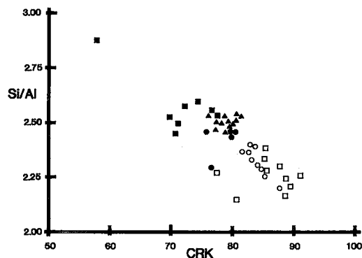
FIG. 4. Si/Al versus CRK [ 100 \times (\text{Cs} + \text{Rb} + \text{K})/\text{cation sum} ] in homogeneous pollucite ( \blacktriangle ), Na-enriched blebs ( \bullet ), Cs-enriched blebs ( \circ ), Na-rich borders of Cs-rich veinlets ( \blacksquare ) and Cs-rich veinlets ( \square ).
