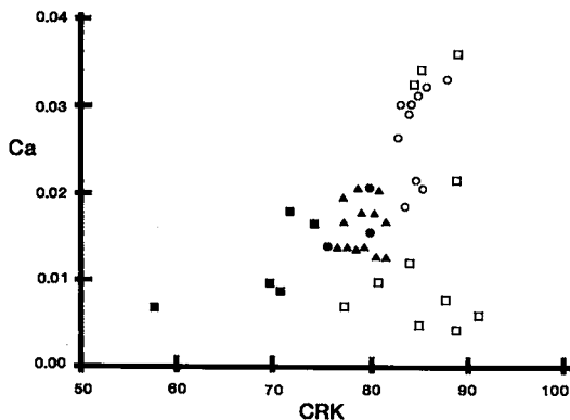
FIG. 7. Ca (atoms p.f.u.) versus CRK [100 \times (Cs + Rb + K)/\text{cation sum}] in homogeneous pollucite, Na-enriched blebs, Cs-enriched blebs, Na-rich borders of Cs-rich veinlets, and Cs-rich veinlets. Symbols as in Fig. 4.
