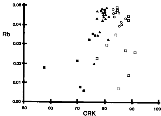
FIG. 6. Rb (atoms p.f.u.) versus CRK [100 \times (Cs + Rb + K)/\text{cation sum}] in homogeneous pollucite, Na-enriched blebs, Cs-enriched blebs, Na-rich borders of Cs-rich veinlets, and Cs-rich veinlets. Symbols as in Fig. 4.
