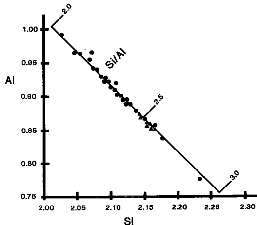
FIG. 3. Al versus Si (atoms p.f.u.) in homogeneous ( \blacktriangle ), and in other textural types ( \bullet ) of pollucite. The homogeneous pollucite has a limited range of Si/Al from 2.45 to 2.55. Data are plotted along the line of best fit (slope 1.00 \pm 0.06 ).
