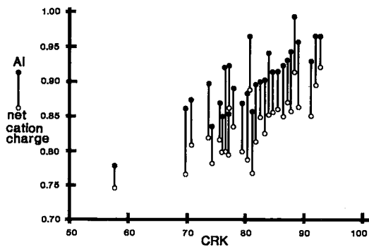
FIG. 9. Al and cation charge sum (atoms p.f.u.) versus CRK [100 \times (Cs + Rb + K)/\text{cation sum}] for High Grade Dyke pollucite. An 8 to 10% deficiency in cationic charges (relative to Al) is seen in each analysis.
