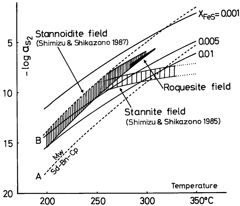
FIG. 5. Temperature - \log a(S_2) diagram for roquesite-bearing ores. Curves A and B correspond to a(S_2) - temperature relationships for the assemblage of stannoidite - chalcopryrite - bornite - mawsonite - S_2(\text{gas}) for a(\text{Fe}) = 1 and a(\text{Fe}) = 0.1 . a(\text{Fe}) is defined as the activity of the \text{Cu}_8\text{Fe}_3^{2+}\text{Fe}^{2+}\text{Sn}_2\text{S}_{12} component in the stannoidite solid solution. Symbols: Mw mawsonite, Sd stannoidite, Bn bornite, Cp chalcopryrite.
