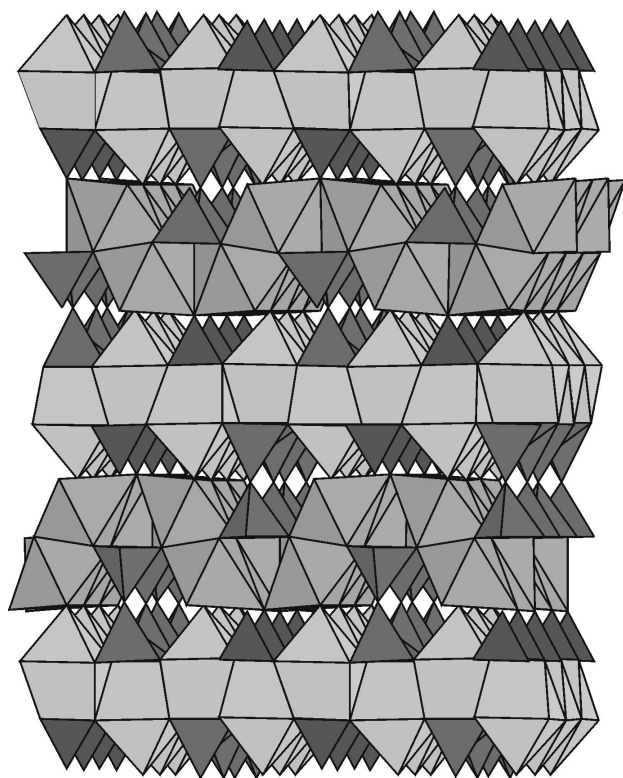
FIGURE 6. Crystal structure of fukalite from Gumeshevsk, MDO1 polytype, as seen down [1\ 0\ 0] , b vertical, with a slight tilt ( -10^\circ ) to give a better view of the structural arrangement.
