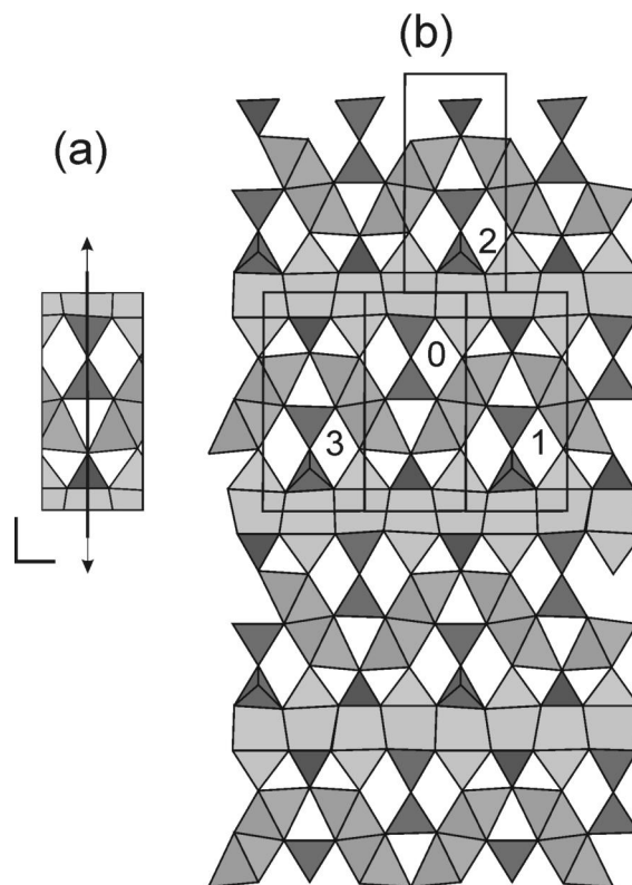
FIGURE 3. (a) Schematic drawing of the rod, with the indication of the symmetry operators; (b) structural model including the four-repeat tetrahedral chains, represented as seen along a , with b horizontal.
