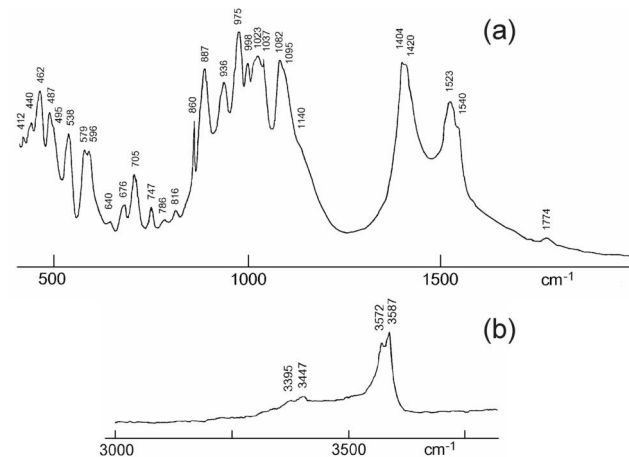
FIGURE 1. IR spectrum of fukalite from the Gumeshevsk deposit.
