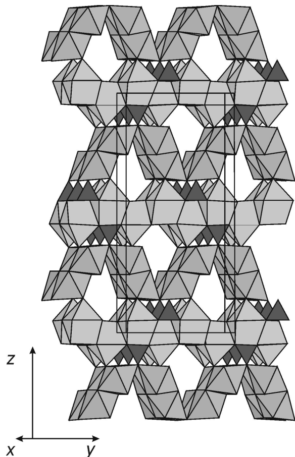
FIGURE 2. The calcium-polyhedron scaffolding as seen down a , with a small tilt ( 10^\circ ) to give a better view of the structural arrangement (data from Rastvetaeva et al. 2005).
