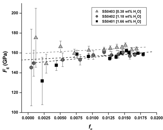
FIGURE 5. Plots of Birch normalized pressure ( F_E ) vs. Euler finite strain ( f_E ) for hydrous wadsleyites. Bulk moduli from y-intercepts of linear regressions are 160(3), 153(3), and 149(3) GPa for samples with 0.38, 1.18, and 1.66 wt% H_2O , respectively. Positive slopes of the linear regressions indicate K' > 4 .
