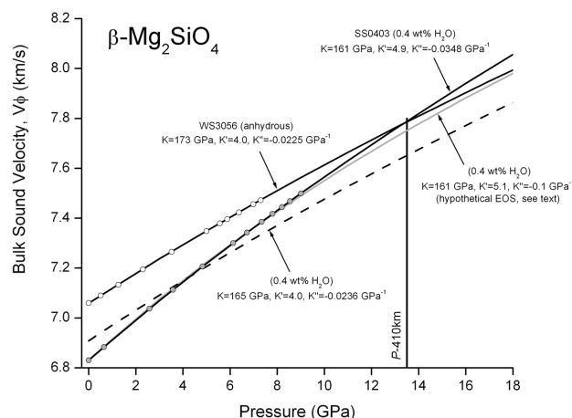
FIGURE 6. Bulk sound speed plots for anhydrous and hydrous wadsleyite (solid black curves), and a hypothetical curve representing possible behavior of hydrous wadsleyite at Transition Zone pressures (gray). Curves are extrapolated from zero-pressure Birch-Murnaghan equation of state parameters; data points represent pressures at which volume data were collected. The dashed curve represents a refit of the hydrous data with K' = 4.0 , consistent with the anhydrous value. The gray curve is calculated from the fitted K_0 and K' , with K'' selected so that bulk sound speeds for the hydrous composition remain lower than the speeds for the anhydrous composition through the pressure stability range of wadsleyite in the Transition Zone. The vertical line represents the approximate pressure at the 410 km seismic discontinuity.
