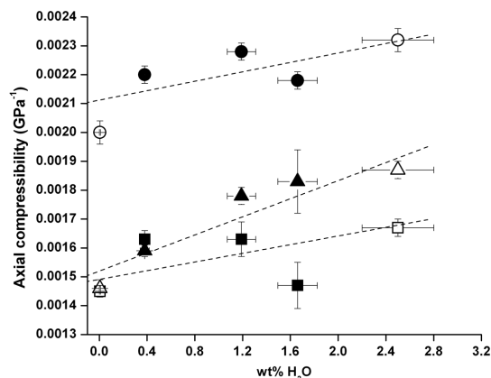
FIGURE 3. Linear compressibility parallel to crystallographic axes for wadsleyite. Squares = a -axis; triangles = b -axis; circles = c -axis. Solid symbols represent the current study; open symbols near 0 wt% are data from Hazen et al. (2000); open symbols at 2.5 wt% are from Yusa and Inoue (1997). Best-fit lines were added to aid in comparing slopes of the data.
