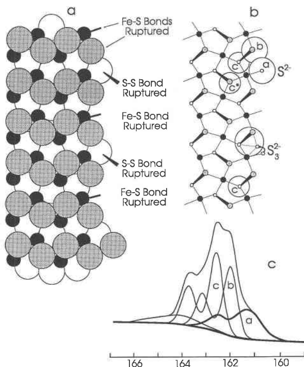
FIGURE 2. Structural and bonding relations in the near-surface region of a pyrite fracture surface, and a XPS S(2p) spectrum of a fractured pyrite surface (modified after Bronold et al. (1994)). (a) Arrangements of S and Fe ions exposed on an atomically rough surface approximately parallel to the {001} plane. Black dots = \text{Fe}^{2+} ions. Shaded circles = S atoms of disulfide situated in a plane immediately "above" the plane containing the Fe ions. Large open circles = S atoms of disulfide located in a plane beneath the plane containing the Fe ions. (b) A ball and stick equivalent of (a). Dots = \text{Fe}^{2+} ions. Disulfide, pairs of patterned and open circles connected by a wedge-shaped line. Patterned circles are situated "above" the Fe plane, and open circles below it. The thick end of the connecting line indicates the "tilt" on the disulfide. Thin straight lines represent Fe-S bonds. The large circle labeled "a" represents the surface states of monosulfide; ("b"), the surface-most S atom of the surface disulfide; ("c"), fully coordinated near-surface S atoms of disulfides; and "c*" S atoms of bulk disulfide. A polysulfide surface state ( \text{S}_2^{2-} ) is also noted. (c) An S(2p) XPS spectrum of a fractured pyrite surface at the bottom of the diagram illustrates the various contributions to the spectrum by the letters, which correspond to the various surface and bulk states of the above ball-and-stick diagram.
