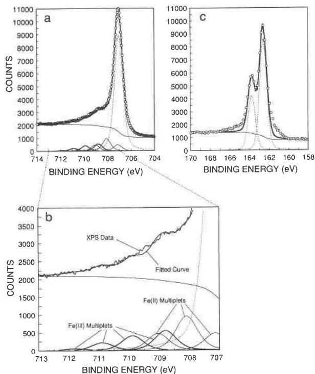
FIGURE 3. High resolution Fe(2p 3/2 ) (a) and S(2p) (c) spectra of vacuum-fractured pyrite. (b) is an expansion of the high-energy tail. Spectrometer settings were 50 eV pass energy and 300 \mu\text{m} X-ray spot size for collection of the spectra. Other instrumental settings and conditions are provided by Splinter et al. (1997). Circles = experimental data. Thick solid curves = the fit to each spectrum. The disulfide doublet is separated by 1.18 eV and both have the same FWHM. The light solid line is the Shirley background.
