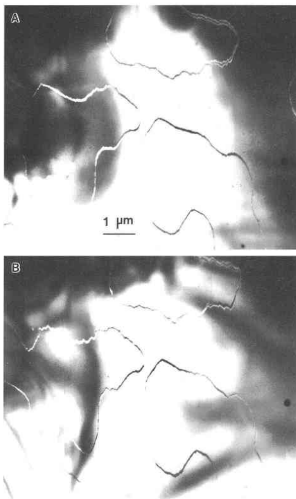
FIGURE 8. Dark-field images of c-APBs. (A) Original configuration; (B) after the specimen was cycled successively about T_c , with \Delta T_0 = 350 °C for 1, 10, 20, 50, 100, 200, 500, 1000, and 2000 s.
