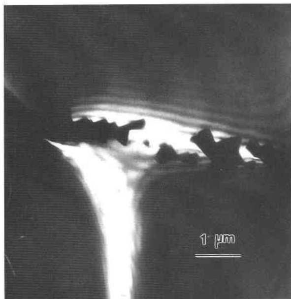
FIGURE 1. Dark-field image of Dauphiné twins. The twins are pinned by the grain boundaries.
