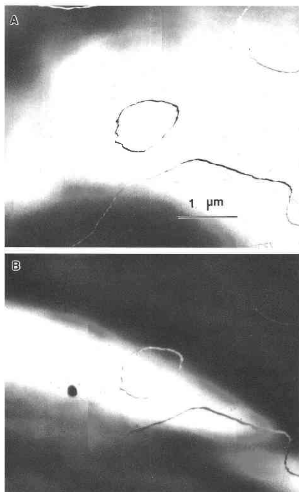
FIGURE 9. Dark-field images of c-APBs. (A) Original configuration; (B) after the specimen was cycled successively about T_c for 10 min, with \Delta T_c = 100, 200, 300, 400, 500, 600 , and 700^\circ\text{C} .
