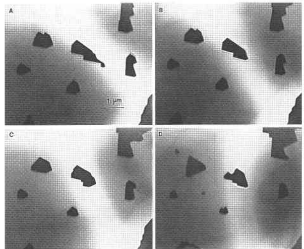
FIGURE 5. Selected dark-field images of Dauphiné twins after the specimen was cycled repeatedly about T_c , with \Delta T_o = 5^\circ\text{C} . (A) Original configuration, (B) annealing time at T_{\max} = 10^\circ\text{C} , (C) 50 s, (D) 200 s.
