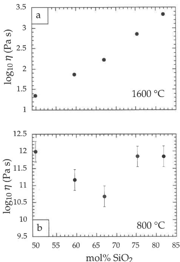
FIGURE 7. Variation of viscosity as a function of silica content at (a) 1600 °C ( T/T_g \approx 1.7 ), and (b) 800 °C ( T/T_g \approx 1 ).
