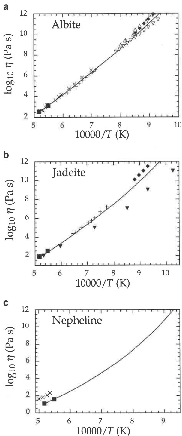
FIGURE 4. Comparison of interpolated viscosity curves (solid line) with literature values, for (a) albite, (b) jadeite, and (c) nepheline. Solid box = Riebling (1966); \times = N'Dala et al. (1984); solid, inverted triangle = Hunold and Brückner (1980); + = Stein and Spera (1993); solid diamond = Taylor and Rindone (1970); open triangle = Hummel and Arndt (1985); open inverted triangle = Cranmer and Uhlmann (1981).
