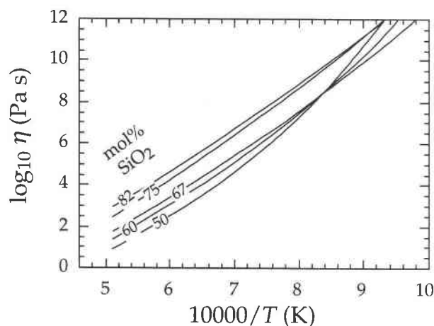
FIGURE 3. Interpolated viscosities of compositions exactly along the join \text{SiO}_2 - \text{NaAlO}_2 .
