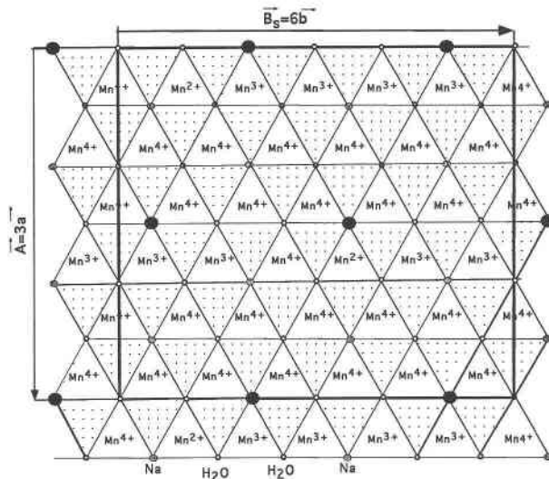
FIGURE 19. Periodic distribution of \text{Mn}^{4+} and \text{Mn}^{2+} along \text{Mn}^{3+} -rich rows in the supercell with A = 3a and B = \lambda = 6b . The periodic distribution of Na (solid circles) and \text{H}_2\text{O} (open circles) with A = 3a and B = 3b supercell parameters is also shown.
