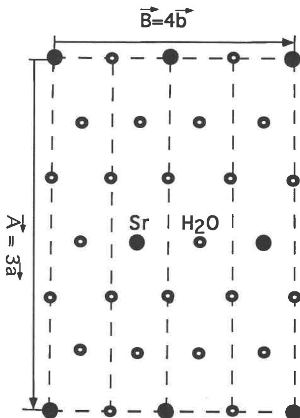
FIGURE 10. A model for the interlayer distribution of Sr (large solid circles) and \text{H}_2\text{O} molecules (small open circles) in SrBi microcrystals with supercell parameters A = 3a and B = 4b .
