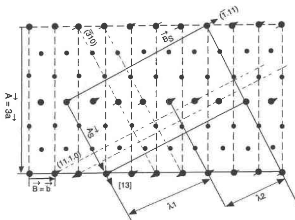
FIGURE 13. A model of the mutual arrangement of Sr (large solid circles) and \text{H}_2\text{O} molecules (small solid circles) in the interlayers of SrBi microcrystals that are characterized by the SAED pattern of Figure 5a. The probability of Sr occupancy is about 0.4–0.45. Arrows show the directions of Sr displacements from their ideal positions. A, B and A_s, B_s are the parameters for the supercell and S cell, respectively. \lambda_1 and \lambda_2 are the wavelengths describing the periodicity of the d_{310} .
