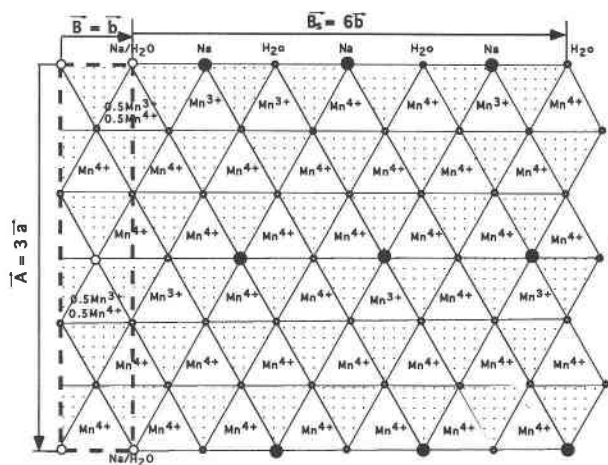
FIGURE 18. Model for the ordered distribution of Na and \text{H}_2\text{O} along b axis, with the sequence Na- \text{H}_2\text{O} -Na- \text{H}_2\text{O} -Na... The rows containing Na and \text{H}_2\text{O} are separated from each other by A/2 along the A axis and are displaced at random by \pm\frac{1}{2} . Na: \text{Mn}^{3+} ratio is 1:6.
