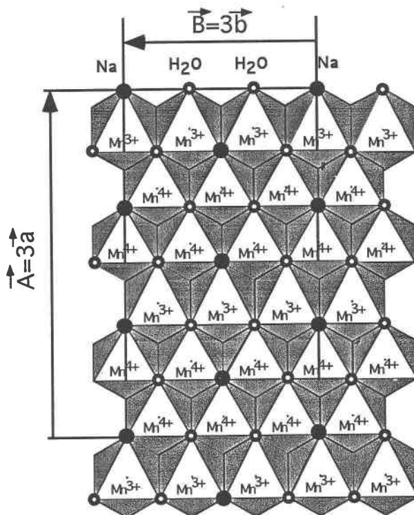
FIGURE 16. Ordered arrangement of \text{Mn}^{3+} and \text{Mn}^{4+} cations among available octahedral sites. A supercell with A = 3a and B = 3b and an ordered distribution of Na (solid circles) and \text{H}_2\text{O} (open circles) is shown.
