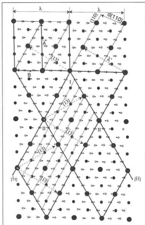
FIGURE 12. Idealized structural model for NaBi interlayers of the second type. Large and small circles represent Na sites with different degrees of occupancy. Small open circles correspond to \text{H}_2\text{O} sites. Arrows attached to circles indicate the periodic displacement of interlayer species along the B axis. In the upper left portion of the diagram two supercells with A = 3a and B = 3b are shown. Unit cells I and II in the form of a rhomb have the same sizes and shapes but differ slightly in the arrangement of Na and \text{H}_2\text{O} sites. \lambda and \lambda' are wavelengths of variation of interplanar distances for (010) and (110), respectively.
