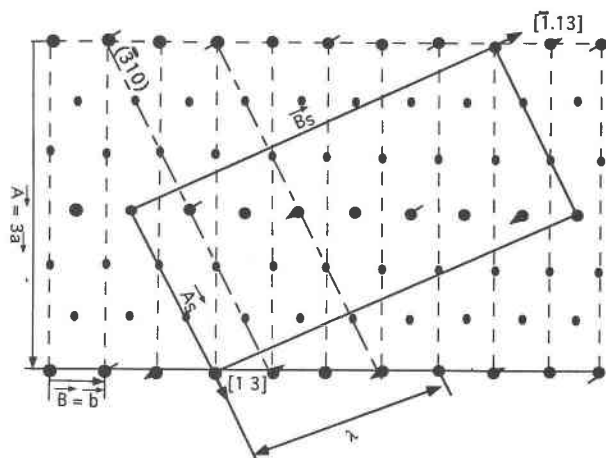
FIGURE 14. A model of the mutual arrangement of Sr (large solid circles) and \text{H}_2\text{O} molecules (small solid circle) in the interlayers of SrBi microcrystals that are characterized by the SAED pattern shown in Figure 5c. The probability of Sr occupancy is about 0.4–0.45. The arrows show the directions of Sr cation displacement in correspondence with the periodic variation of d_{310} . A, B and A_s, B_s are the parameters of the supercell and S cell, respectively.
