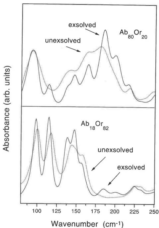
FIGURE 8. Spectral differences between exsolved and uniform samples in the region between 80 and 250\text{ cm}^{-1} for two chemical compositions ( Q_{od} \approx 1 ).
