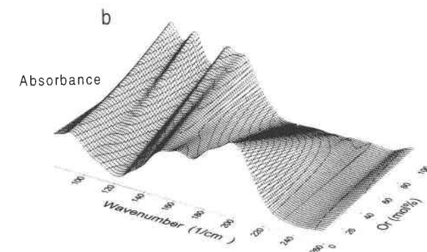
FIGURE 2. Secondary reference spectra in the region between 80 and 260 \text{cm}^{-1} : (a) Q_{\text{od}} \approx 1 , (b) Q_{\text{od}} \approx 0 . The effect of concentration variations on the heights of the 113 and 184 \text{cm}^{-1} bands and the spectral features in this region are used for the determination of chemical composition.
