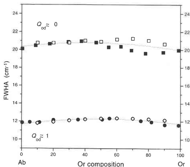
FIGURE 7. Linewidth of the IR band at 640\text{ cm}^{-1} as a function of composition for Q_{od} \approx 1 and Q_{od} \approx 0 . The solid symbols are data from primary reference samples (unexsolved feldspars); the open symbols are data from secondary reference spectra (exsolved feldspars). The average errors for linewidths are 0.25\text{ cm}^{-1} for ordered samples and 1.0\text{ cm}^{-1} for disordered samples.
