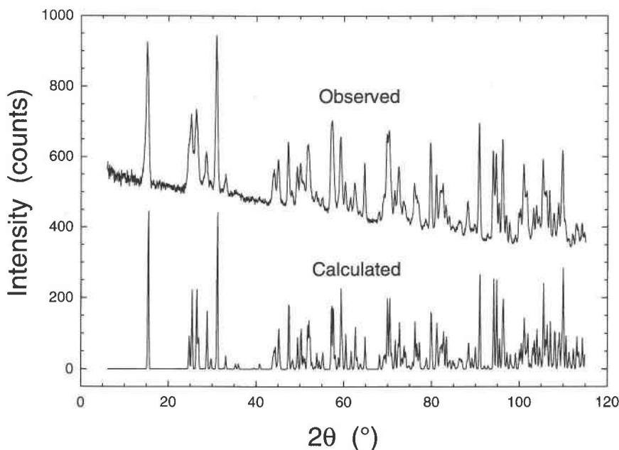
FIGURE 5. Comparison of neutron powder diffraction patterns obtained for the Keokuk kaolinite (observed) with that calculated for the LDF-optimized kaolinite structure. The difference in intensities between the two patterns is related to the background counts associated with the neutron diffraction experiment. No background correction was made so as to preserve the offset between patterns.
