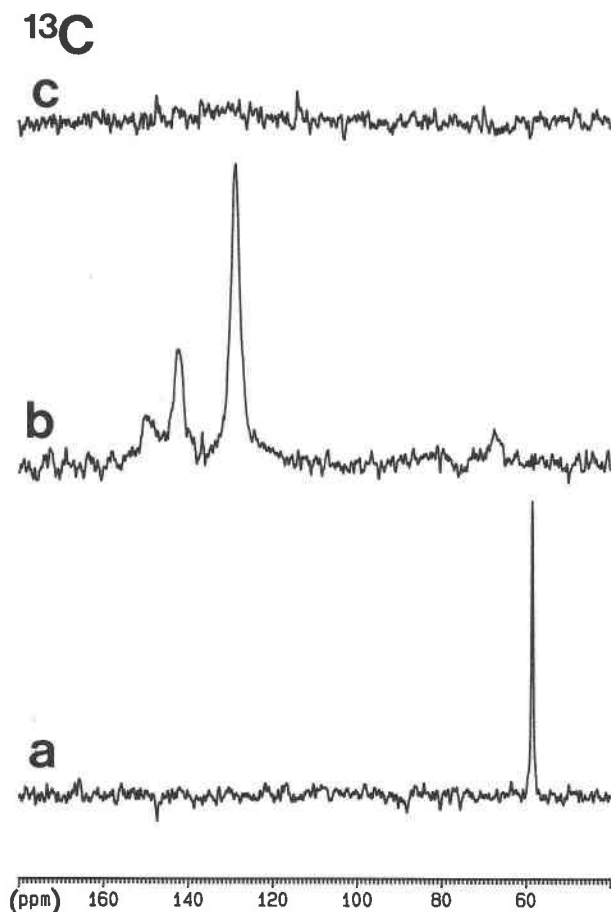
FIGURE 4. The ^{13}\text{C} CP MAS NMR spectra of tsaregorodtsevite (a) unheated (383 scans), (b) heated at 690 °C (1703 scans), and (c) heated at 970 °C (10 971 scans).
