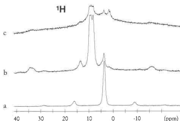
FIGURE 5. The ^1\text{H} MAS NMR spectra of tsaregorodtsevite, (a) unheated, (b) heated at 690 °C, and (c) heated at 970 °C.
