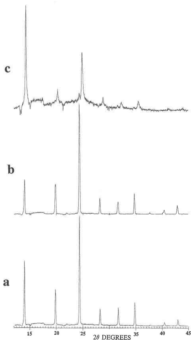
FIGURE 3. Powder XRD patterns of tsaregorodtsevite (a) unheated, (b) heated at 690 °C, and (c) heated at 970 °C.
