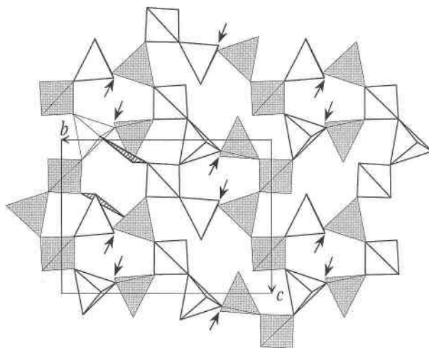
FIGURE 6. Projection of an \text{Si}_6\text{O}_{13} layer present in the framework silicate \text{K}_2\text{CeSi}_6\text{O}_{15} (Karpov et al. 1976), along a direction normal to (100). Unshaded tetrahedra are upward directed, whereas those that are shaded are downward directed. Arrows indicate the locations of the bridging O atoms at which the layer is linked to others (not shown) to form a three-dimensional structure. Hatched triangles correspond to the faces of two distinct \text{CeO}_6 octahedra, one above the plane of the layer and one below.
