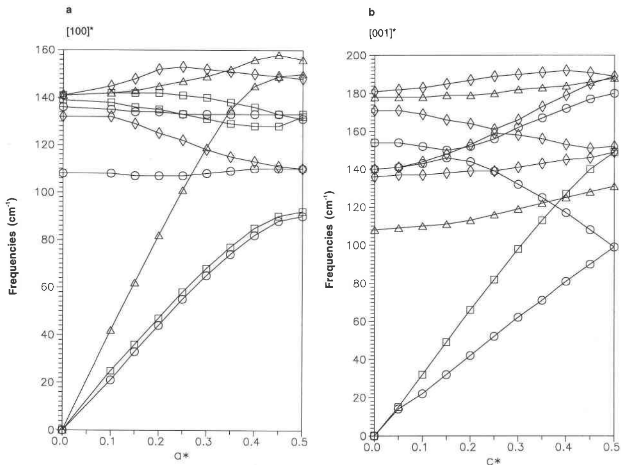
FIGURE 1. Lower branches of calculated phonon dispersion curves for beryl along [100]* (a) and [001]* (b). Different symbols refer to different symmetry representations ( \Sigma_1 - \Sigma_4 and \Delta_1 - \Delta_4 , respectively).
