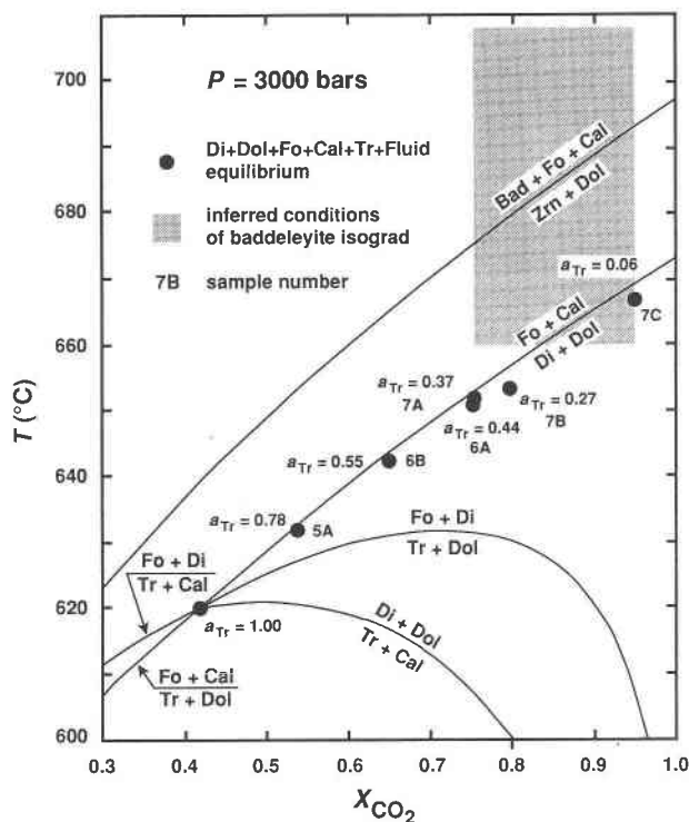
FIGURE 3. T - X_{\text{CO}_2} diagram depicting phase equilibria among diopside (Di), dolomite (Dol), forsterite (Fo), calcite (Cal), tremolite (Tr), zircon (Zrn), baddeleyite (Bad), and \text{CO}_2 - \text{H}_2\text{O} fluid at 3 kbar calculated from Berman's (1988) data base, updated August 1990. All minerals except Cal and Tr are assumed to be pure substances. Cal compositions were adjusted for equilibrium with Dol. Solid circles represent T - X_{\text{CO}_2} conditions estimated for six occurrences of the assemblage Di + Dol + Fo + Cal + Tr with reduced Tr activity ( a_{\text{Tr}} ) as indicated; unit Tr activity assumed along calculated curves. Conditions of the baddeleyite isograd predicted by the Zrn + Dol + Bad + Fo + Cal equilibrium are consistent with independently inferred conditions based on other mineral-fluid equilibria (shaded rectangle).
