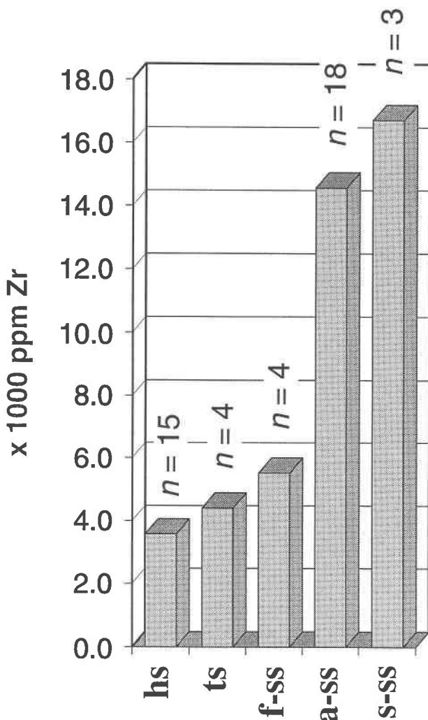
Fig. 2. A histogram showing the average whole-rock content of Zr in the principal varieties of granite at Strange Lake. Abbreviations: hs = hypersolvus, ts = transsolvus, f-ss = fresh subsolvus, a-ss = altered subsolvus, and s-ss = strongly altered subsolvus. Standard deviations are 1.9, 2.4, 1.3, 2.3, and 0.3 \times 1000 ppm, respectively.
