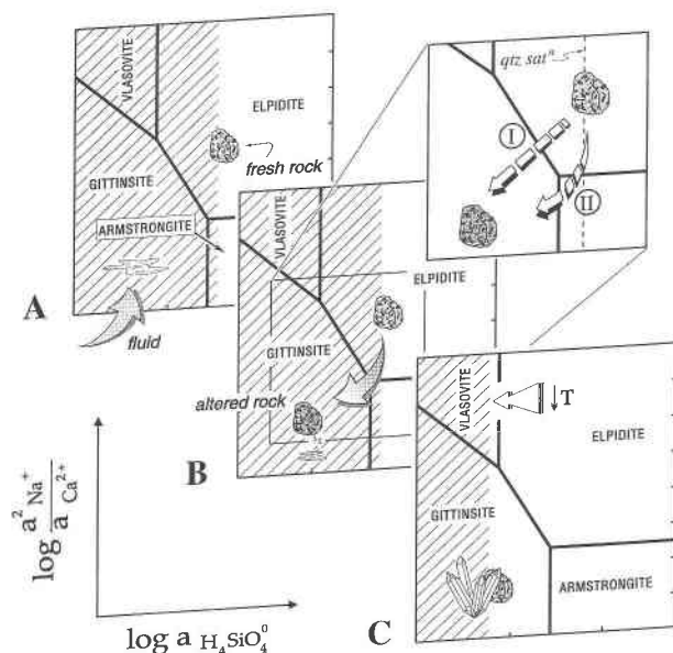
Fig. 7. Schematic \log a_{Na^+}/a_{Ca^{2+}} vs. \log a_{H_4SiO_4^0} diagrams showing the stability fields of the zirconosilicate minerals, as well as hypothetical compositions of the unaltered elpidite-bearing granite, the hydrothermal fluid (A), and the altered gittinsite-bearing granite (C). Also shown are possible paths of metasomatic transformation of the rock during alteration (B). The shaded fields represent quartz saturation levels in the fluid during metasomatism (A and B) and at lower temperature (C).
