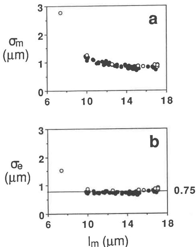
Fig. 3. (a) Conventional standard deviation ( \sigma_m ) vs. arithmetic mean fission track length ( l_m ). (b) Elliptical standard deviation ( \sigma_e ) vs. arithmetic mean fission track length ( l_m ). Typical 2\sigma error bar for l_m is approximately as wide as the symbols used. Solid symbols, Q \geq 0.05 ; open symbols, Q < 0.05 .
