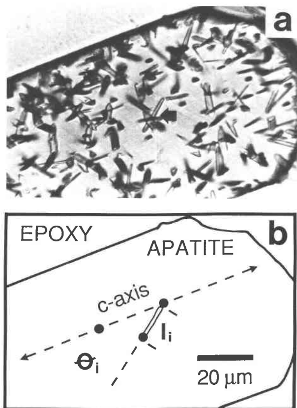
Fig. 1. (a) Photomicrograph of a horizontal confined fission track, indicated by the arrow, in Tioga apatite. (b) Schematic representation of a with the crystallographic c-axis indicated and the three points, indicated by solid dots, used for track length ( l_i ) and orientation ( \theta_i ) measurement.
