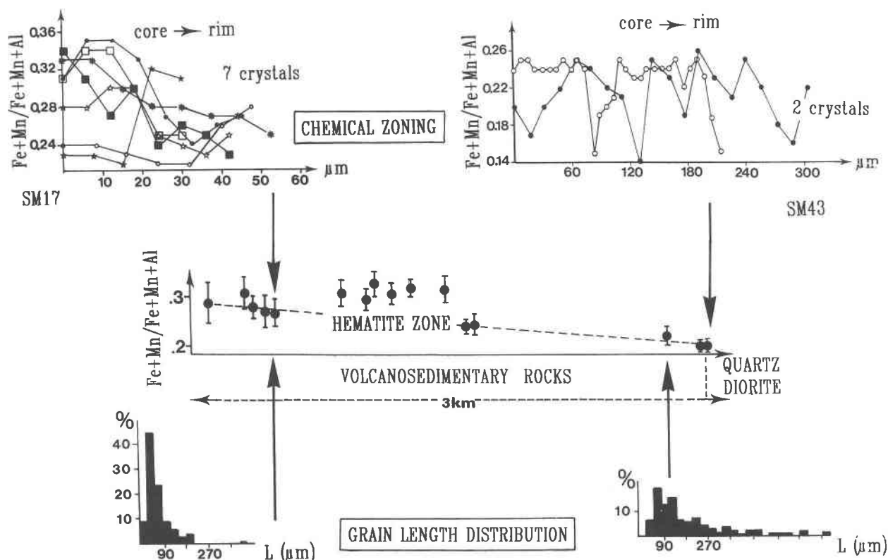
Fig. 3. Chemical composition of epidote samples as well as their compositional variations, expressed by \text{Fe} + \text{Mn}/\text{Fe} + \text{Mn} + \text{Al} atomic ratio (average values and standard deviations), plotted in terms of distance from the quartz-diorite pluton. In the hematite zone, where the epidote + chlorite + hematite paragenesis is encountered (i.e., in Fe cherts), the X_{\text{Fe}} ratio is close to 0.33.
