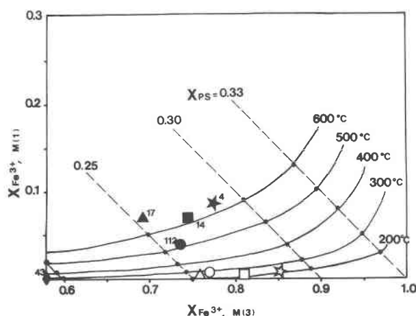
Fig. 5. Theoretical distribution of \text{Fe}^{3+} in M1 and M3 sites in epidote, determined by Bird et al. (1988) from Bird and Helgeson (1980). Solid symbols = observed values for the investigated samples; open symbols = theoretical values for the same samples denoted by the solid symbols.
