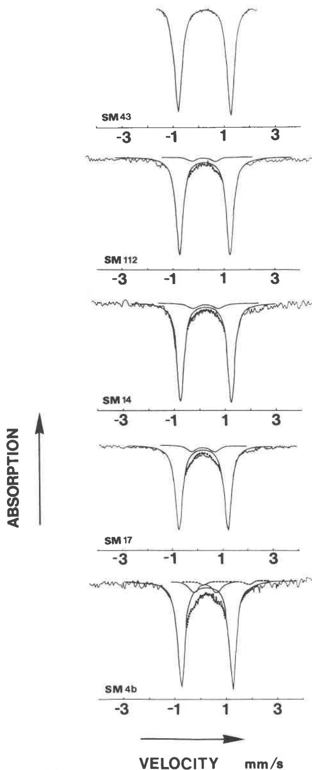
Fig. 4. Mössbauer spectra of the epidotes studied. Solid curves = doublets attributed to \text{Fe}^{3+} in M3 and M1 sites. Dashed curves = doublet attributed to \text{Fe}^{2+} . Circles = calculated fit. For sample SM4, only the best fitted deconvolution, taking the \text{Fe}^{2+} signal into account, is depicted (sample 4b).
