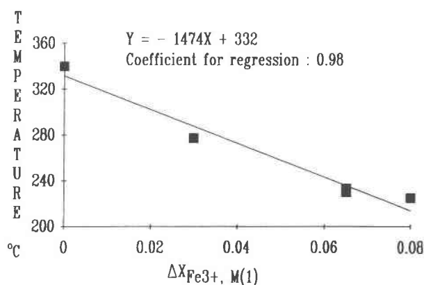
Fig. 6. Deviation from equilibrium theoretical values ( \Delta X_{\text{Fe}^{3+}, \text{M}(1)} ) as a function of the temperature that affected the samples during epidote crystallization.
