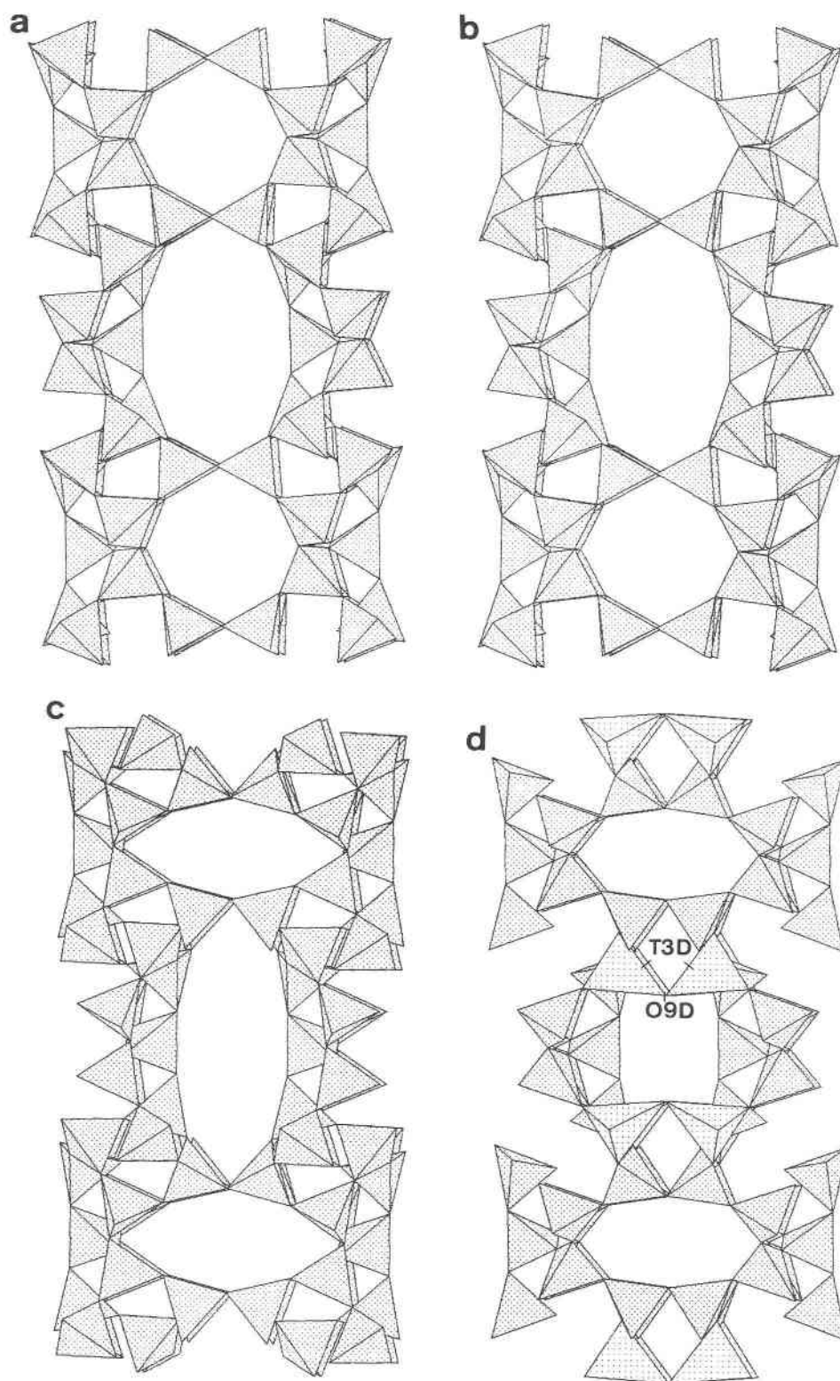
Fig. 3. Projection inclined 2^\circ from [001] displaying the tetrahedral framework at various degrees of dehydration. (a) Natural sample; (b) dehyd2 sample; (c) dehyd4 (heat-collapsed) sample; (d) sample Nadap, phase B (Alberti and Vezzalini, 1983).
