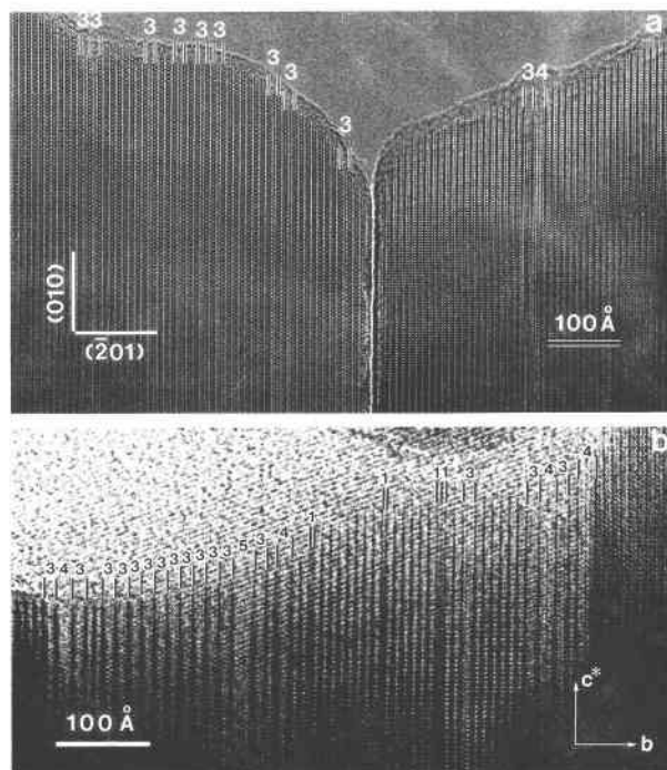
Fig. 6. TEM images of synthetic tremolite containing wide-chain defects. (a) Two neighboring crystals in Tr5-18 vary significantly in defect density. The crystal on the left contains more wide-chain slabs (mainly triple-chain structures, labeled 3) than the one on the right. (b) A highly disordered crystal containing a slab with ten contiguous triple-chain slabs (Tr1-21). Single-, quadruple-, and quintuple-chain structures (labeled 1, 4, and 5, respectively) are also intergrown.
