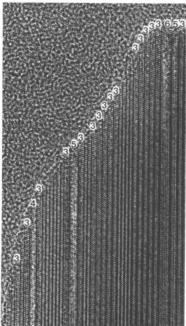
Fig. 7. The (0 kl ) lattice-fringe images from a crystal consisting mainly of triple chains and other wider-chain pyroble structures (Tr2).
