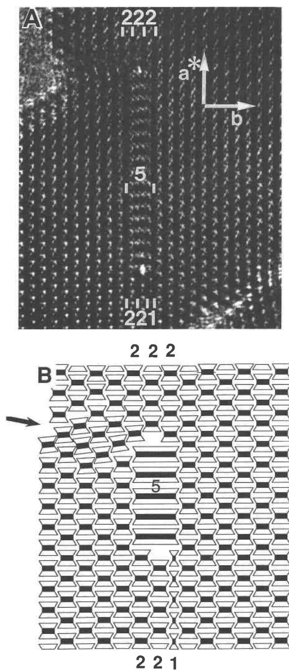
Fig. 5. (A) HRTEM image of an intergrowth of a single chain within crocidolite. The single chain occurs where a quintuple chain (5) terminates to two double chains plus a single chain (221). The quintuple chain also terminates incoherently to three double chains (222). (B) A schematic I-beam model showing the features in A; the arrow points to a disrupted region resulting from the structural mismatch. The termination of a quintuple-chain slab producing a single-chain slab is consistent with the out-of-phase boundary model of Veblen and Buseck (1981).
