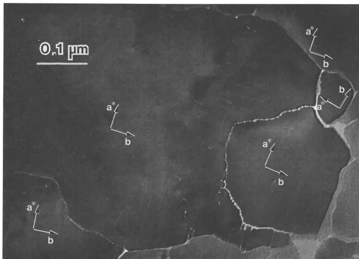
Fig. 3. Low-magnification image of a relatively large crocidolite crystal, the edge of which shows the development of smaller crystals having similar orientations. The small crystals have irregular grain boundaries. The large crystal contains abundant defects that result in white contrast in the image.
