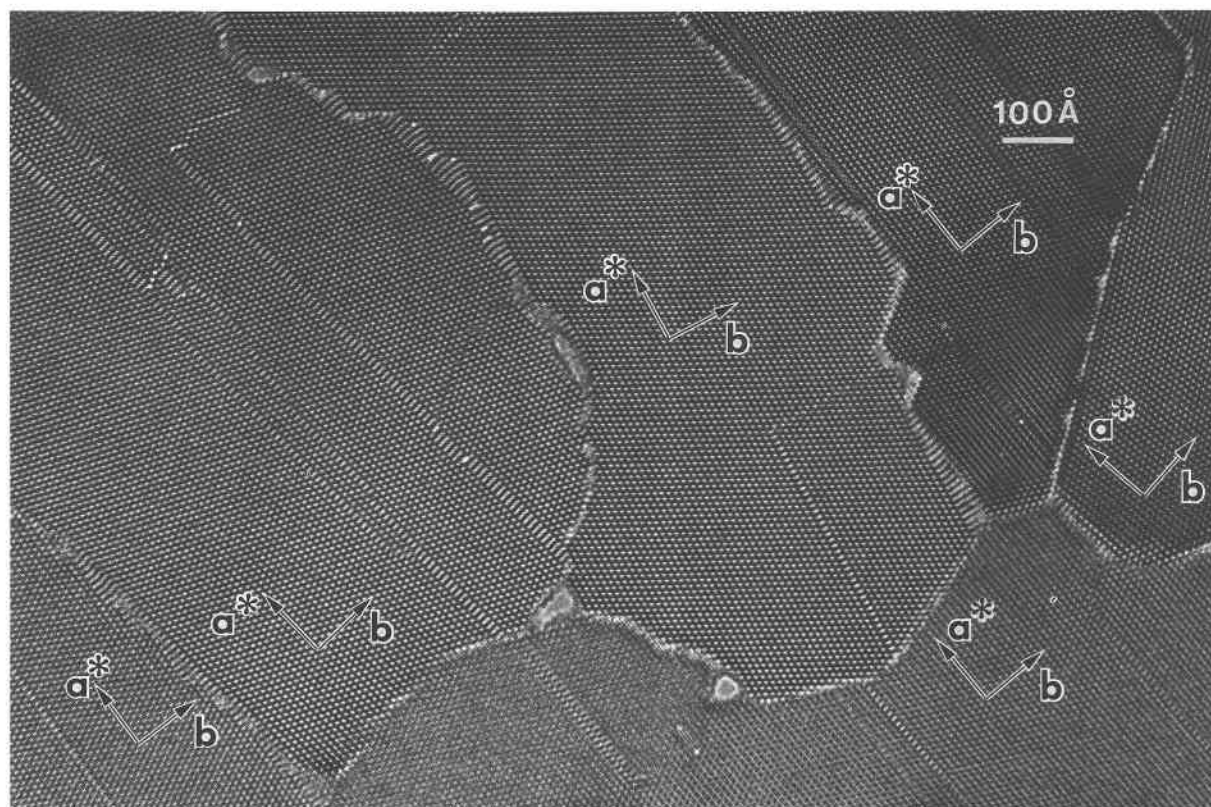
Fig. 13. A crystal that was polygonized to slightly rotated subgrains. Chain-width errors and zipper terminations are common within the subgrains. The (010) boundaries are relatively well defined, and the gaps between (010) boundaries of adjacent subgrains are filled by wedge-shaped masses of wide-chain biopyriboles. Boundaries having other orientations are not as well defined.
