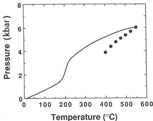
Fig. 9. P - T diagram illustrating the uplift path delineated by Hall et al. (1991) for Ducktown rocks (line) and the calculated P - T path (pseudoisochore) traversed by hypothetical peak metamorphic fluid inclusions during cooling (dots).
