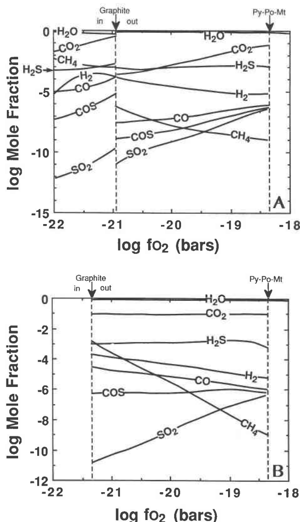
Fig. 5. X_i - f_{O_2} relations calculated for 6 kbar and 550 °C with f_{O_2} and f_{S_2} constrained by trend A (Fig. 3). (A) The a_c = 0.001 above log f_{O_2} of -20.96 , which produces a maximum X_{CO_2} of 0.3. (B) X_{CO_2} = 0.10 ( a_c = 1 - 0.001 ). The graphite maximum is located at f_{O_2} = -21.35 , which corresponds to a X_{CO_2} of 0.1.
