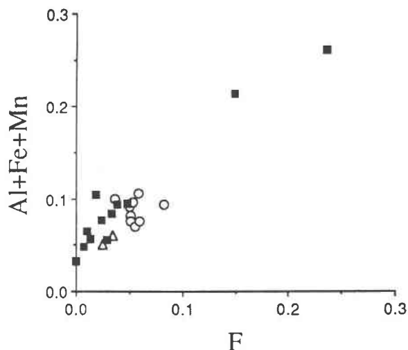
Fig. 8. Plot of \text{Al} + \text{Fe} + \text{Mn} vs. \text{F} in ion numbers per formula unit for titanite from the Tananao orthogneiss (open symbols), including intergranular titanite (circles) and titanite replacing ilmenite inclusions in biotite (triangles). The positive trend is more obvious when the analyses of titanite compiled by Higgins and Ribbe (1976) are also plotted (solid squares).
