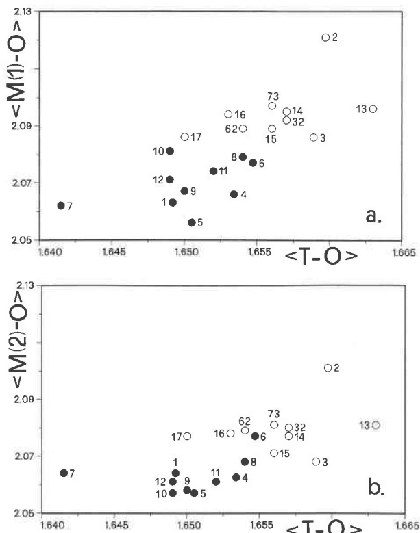
Fig. 7. Mean \langle M-O \rangle distance ( \text{\AA} ) vs. mean \langle T-O \rangle distance ( \text{\AA} ) for M1 (a) and M2 (b). Symbols and samples as in Figure 1.
