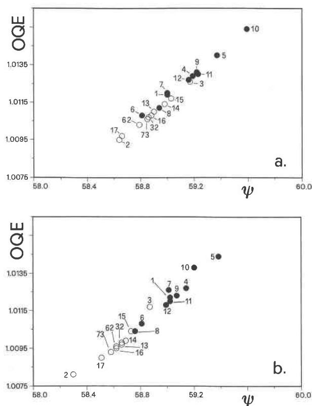
Fig. 2. OQE vs. \psi (°) for M1 (a) and M2 (b) sites. Symbols and samples as in Figure 1.
