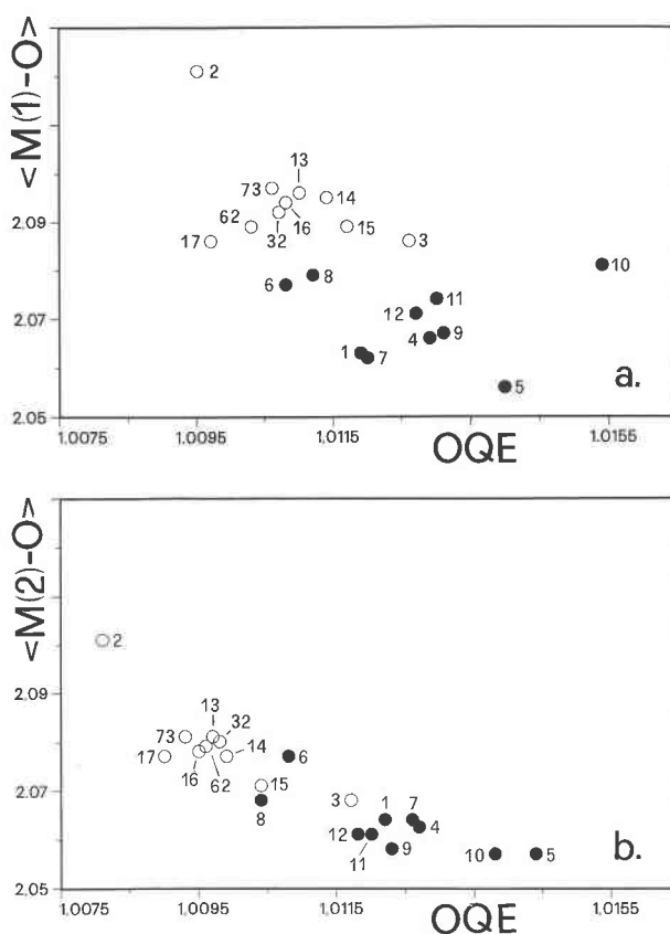
Fig. 3. Mean \langle M-O \rangle distance (Å) vs. OQE for M1 (a) and M2 (b) sites. Symbols and samples as in Figure 1.
