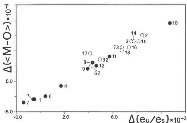
Fig. 4. Values of \Delta\langle M-O \rangle = (\langle M1-O \rangle - \langle M2-O \rangle) (Å) vs. \Delta(e_u/e_s) = (e_u/e_s)_{M1} - (e_u/e_s)_{M2} . Symbols and samples as in Figure 1.
