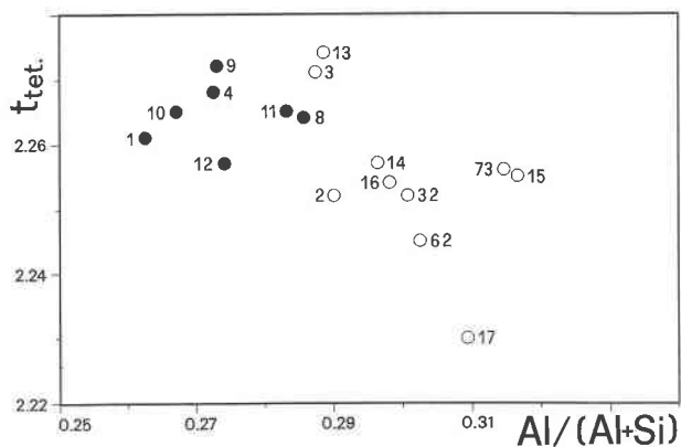
Fig. 6. Values of t_{tet} vs. Al/(Al + Si) . Symbols and samples as in Figure 1.
