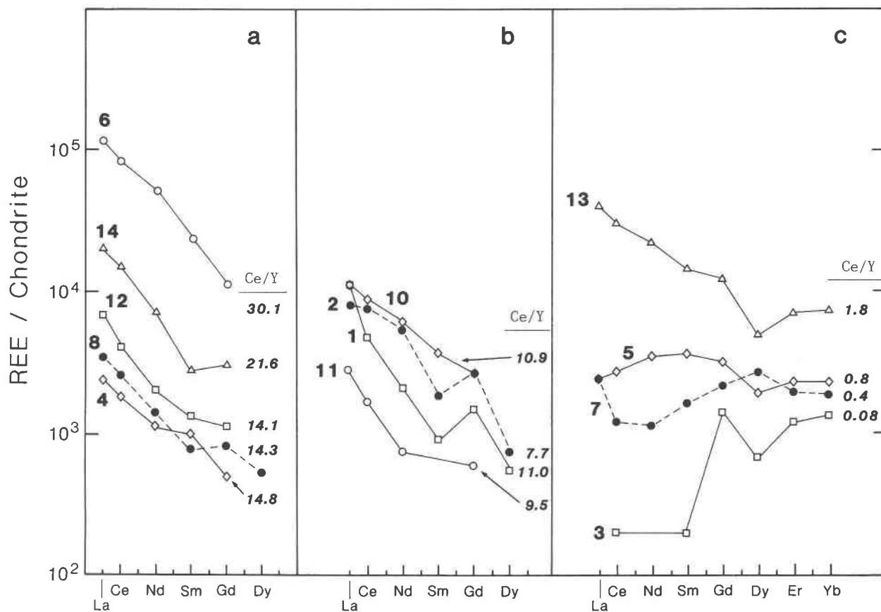
Fig. 2. REEs in apatite normalized to the distribution found in a chondritic meteorite. The sample number is shown in bold type to the left of each curve and the Ce/Y ratio is shown to the right of each curve.
