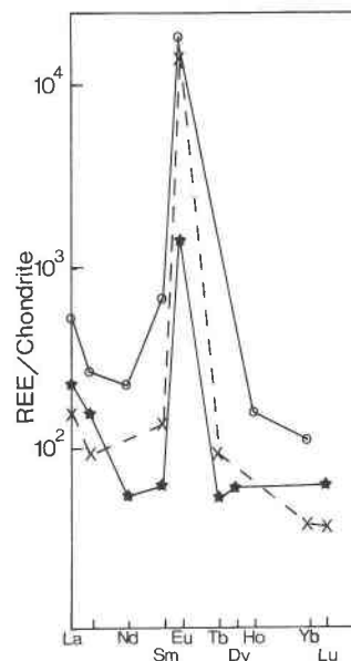
Fig. 6. REEs normalized to the REE content found in a chondritic meteorite for the Llallagua apatite as determined by PIXE (circles) and by neutron activation (crosses) and for the Panasqueira apatite (stars) as reported by Knutson et al. (1985).
