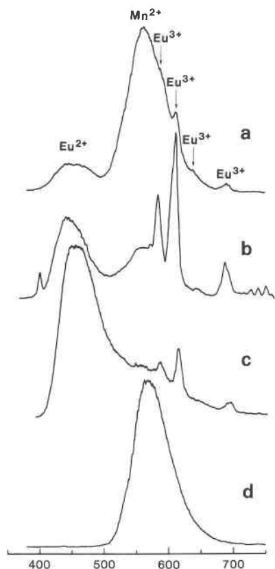
Fig. 4. (a) Cathodoluminescence and (b) ultraviolet-induced spectra for the Llaguna apatite (sample 9) plotted from 400 to 700 nm. Spectrum (c) is of an apatite doped with Eu and synthesized at low oxygen fugacity. Spectrum (d) is of a synthetic apatite doped with Mn.
