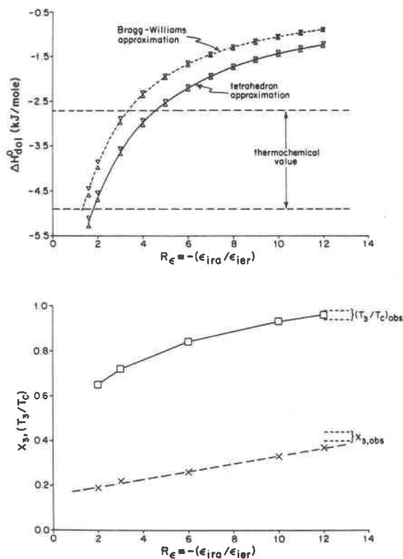
Fig. 3. (a) The enthalpy of stabilization of dolomite, \Delta H^\circ_{\text{dol}} , as a function of R_e ( R_e = -\epsilon_{\text{ira}}/\epsilon_{\text{ier}} ). The horizontal dashed lines indicate the thermochemical value ( \Delta H^\circ_{\text{dol}} = 3.8 \pm 1.1 kJ/mole from Robie et al. , 1979); the solid curve gives calculated values for the tetrahedron approximation; and the dashed curve gives calculated values for the Bragg-Williams approximation. Note that for a fixed value of T_c , the tetrahedron approximation always gives a lower value for \Delta H^\circ_{\text{dol}} than the Bragg-Williams approximation. (b) The quantities (T_3/T_c) and X_3 as functions of R_e . Note that a value of R_e \approx 12 is required for agreement with the experimental diagram, as opposed to the value 2 \leq R_e \leq 4.5 that is indicated by Fig. 3a.
