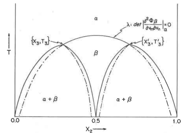
Fig. 1. Idealized phase diagram for \text{CaCO}_3\text{-MgCO}_3 and related systems. Phase \alpha is a high-temperature higher symmetry phase and \beta is a low-temperature lower symmetry phase. The curve- \lambda is a line of higher than first-order transition which, if second-order, is defined by the condition \det[\partial^2 \phi_{\text{ord}} / \partial v_m \partial v_n]_{\text{dis}} = 0 , where v_m and v_n define the state of LRO. Dot-dashed extensions of \lambda are the ordering spinodals (as in Allen and Cahn, 1976). \{X_3, T_3\} and \{X_3', T_3'\} are tricritical points below which the stability field for \beta is flanked by two phase fields.
