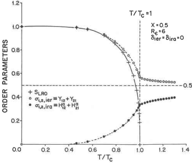
Fig. 4. The long-range order parameter ( S_{LRO} = crosses), and two short-range order parameters, \sigma_{12,ier} \equiv Y_{12} + Y_{21} (open circles) and \sigma_{12,ira} \equiv H_{12}^a + H_{21}^a (closed circles), as functions of reduced temperature ( T/T_c ) for X = 0.5 and R_e = 6 . Note that above T/T_c = 1 both SRO parameters deviate significantly from the random distribution value of 0.5; also note that \sigma_{12,ier} deviates far less than \sigma_{12,ira} because the absolute value of \epsilon_{ier} is a factor of six smaller than the absolute value of \epsilon_{ira} .
