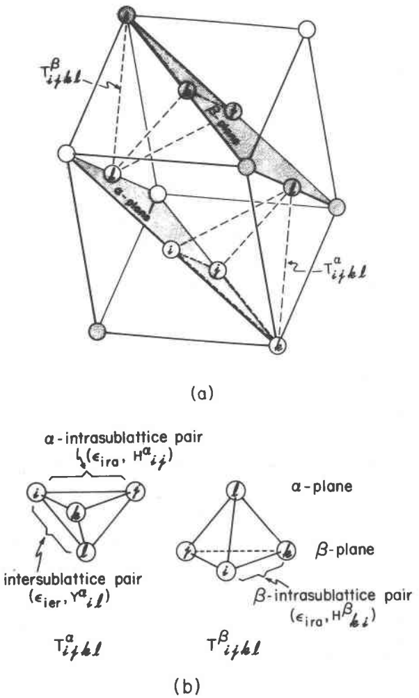
Fig. 2. (a) Schematic drawing of a trigonally distorted fcc lattice with alternating \alpha and \beta planes. (b) Tetrahedron basic clusters corresponding to the distribution variables T^{\alpha}_{ijkl} and T^{\beta}_{ijkl} ; also indicating the energy parameters and sublattice distribution variables associated with intersublattice ( \epsilon_{ier}, Y^{\alpha}_{ij} ) and intrasublattice ( \epsilon_{ira}, H^{\alpha}_{ij} ) near neighbor pairs.
