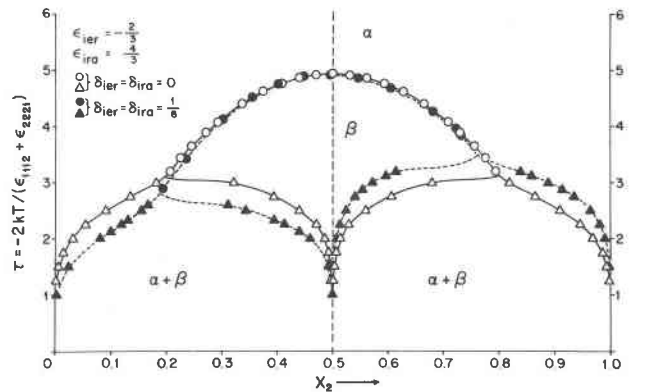
Fig. 5. The solid line (with open symbols) indicates the symmetric diagram calculated with R_e = 2 and \delta_{ier} = \delta_{ira} = 0 . The dashed line (with closed symbols) gives the asymmetric diagram for R_e = 2 , \delta_{ier} = \delta_{ira} = -\epsilon_{ier}/4 . Note the effect of \delta_{ier} and \delta_{ira} on T_3 and T_3' .
