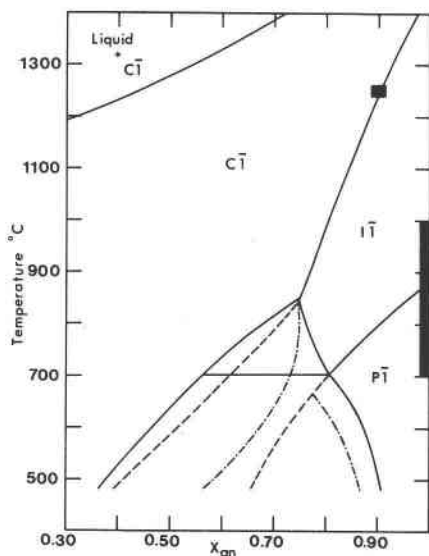
Fig. 8. Proposed temperature-composition diagram for the calcic portion of the system anorthite-albite. Temperature of the C\bar{1} \rightleftharpoons \bar{I}\bar{1} transition for An_{90} is inferred from TEM observations of Nord et al. 1973. The temperature of the \bar{I}\bar{1} \rightleftharpoons P\bar{1} transition is uncertain and may lie within the range of temperatures ( 1000^\circ – 700^\circ\text{C} ). Dashed lines are metastable extensions of the higher-order transitions within the miscibility gaps. Dash-dot lines are the traces of the spinodals on the free energy curve of the low symmetry phases. The positions and temperatures of the tricritical points are inferred from TEM observations.
