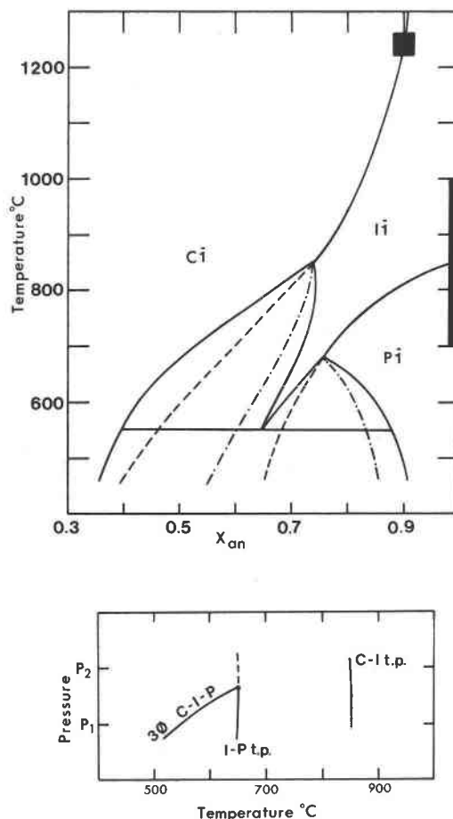
Fig. 9. (a) A possible topology of the temperature-composition diagram for the calcic portion of the system albite-anorthite. This version contains a region of stability for the \bar{I}\bar{1} – P\bar{1} conditional spinodal. Compare with Fig. 8. (b) Pressure-temperature relations for the univariant equilibrium P\bar{1} + \bar{I}\bar{1} + C\bar{1} ( 3\phi C – I – P ) and the two tricritical points; C\bar{1} – \bar{I}\bar{1} ( C – I t.p.) and \bar{I}\bar{1} – P\bar{1} ( I – P t.p.). The T – X diagram above corresponds to an isobaric section at P_1 . The T – X diagram in Fig. 8 would correspond to an isobaric section at P_2 , a pressure above the invariant point terminal to the C\bar{1} – \bar{I}\bar{1} – P\bar{1} univariant reaction. The \bar{I}\bar{1} – P\bar{1} tricritical point is metastable under these conditions. Temperatures are approximate and pressure increases from P_1 to P_2 .
