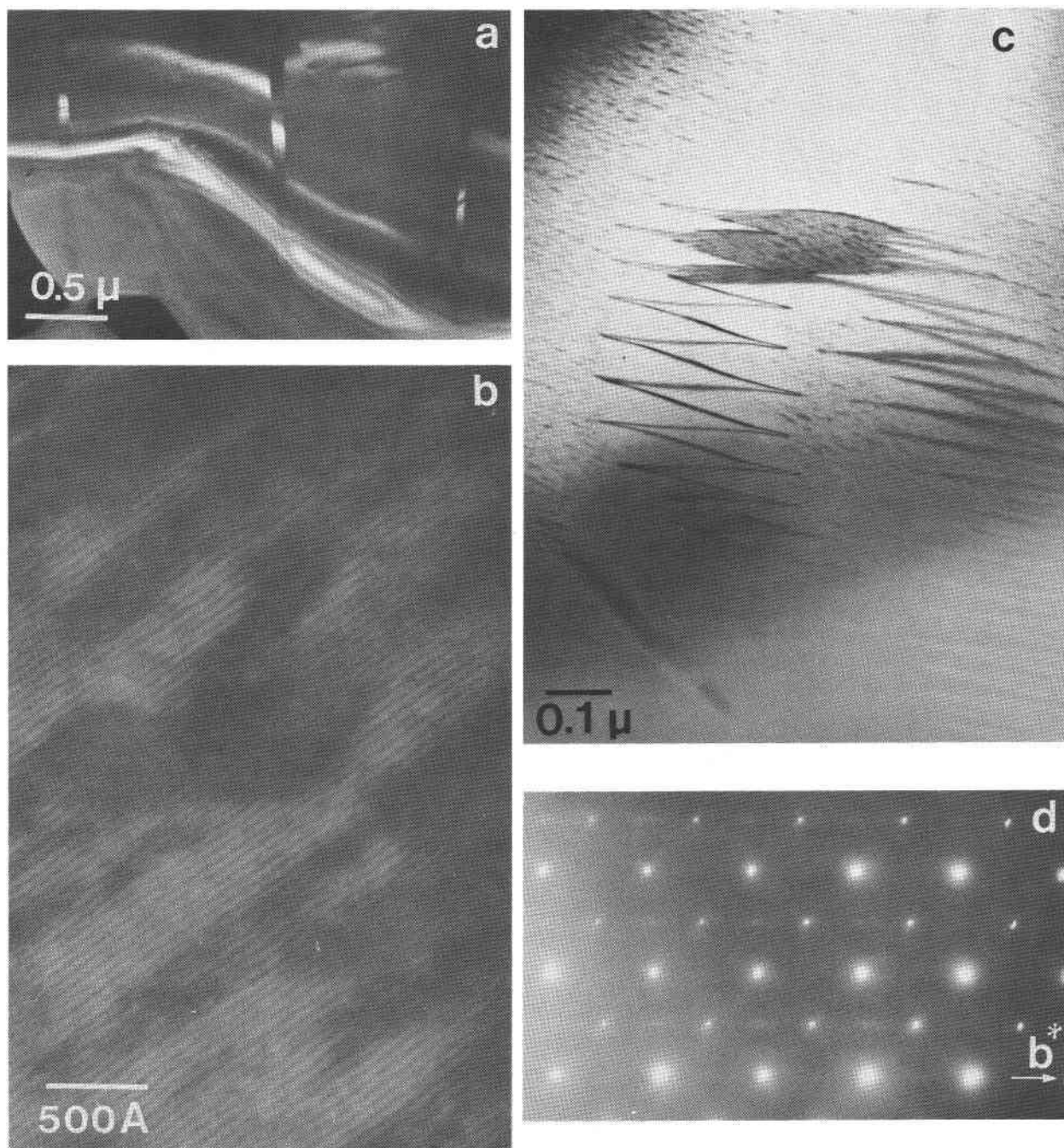
Fig. 10. TEM observations of plutonic plagioclase. (a) Nain plagioclase An_{66-70} contains isolated lamellae of the calcic phase. DF, g = 013 . (b) Nain labradorite An_{72} . Two phase intergrowth of C\bar{1} and I\bar{1} formed by cooling into the conditional spinodal from the stability field of C\bar{1} . Ordering on I\bar{1} produces APBs, which on decomposition are wetted by the C\bar{1} phase. Because the I\bar{1} periodic antiphase domains overlap, it is not possible to see the regions of C\bar{1} . Light regions are inferred to be I\bar{1} , dark regions are inferred to be C\bar{1} . DF, g = 02\bar{2} . (c) Stillwater bytownite An_{82} . Zigzag b APBs have served as sites for heterogeneous nucleation of C\bar{1} phase. The C\bar{1} phase has transformed to the periodic antiphase structure as seen by the periodicity on the APB (upper center). Within I\bar{1} ordered domains metastable P\bar{1} and I\bar{1} decomposition has occurred. Regions adjacent to the APB are devoid of these precipitates. DF, g = 031 . (d) [100] selected area diffraction pattern of Stillwater bytownite. The diffuse c reflections indicate P\bar{1} symmetry. b^* is horizontal and c^* is vertical.
