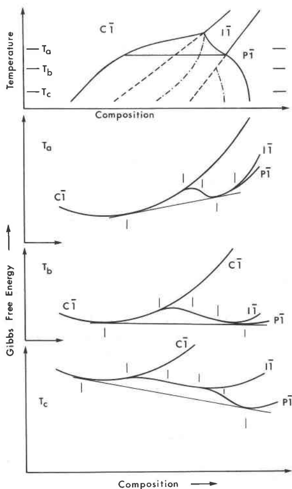
Fig. 11. Free energy ( G )-composition diagrams show possibilities for metastability. For selected isotherms on the schematic T - X diagram G - X diagrams are constructed below. T_a shows G - X curves at a temperature below the C\bar{1} - I\bar{1} tricritical point. T_b shows G - X curves above the P\bar{1} - I\bar{1} tricritical point, but below the intersection of the P\bar{1} stability field with the two-phase region. T_c shows G - X curves at a temperature below both tricritical points. Tangent planes show the equilibrium compositions of two-phase assemblages that define the miscibility gap. Vertical marks below the tangent surface emphasize the compositions. Vertical marks above the G -curves show the stable and metastable transition points and spinodals.
