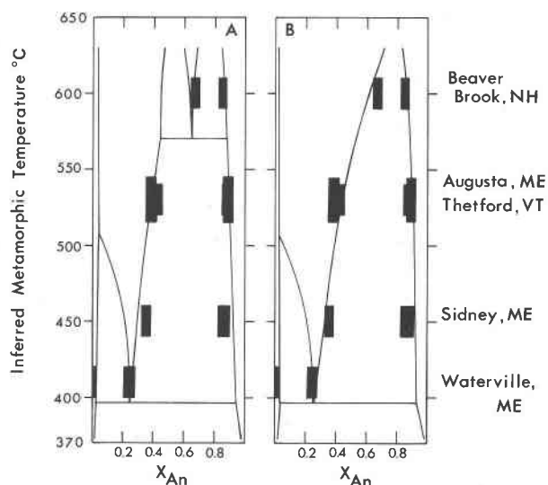
Fig. 1. Electron microprobe analyses of plagioclase from metamorphic rocks. The dark rectangles represent preferred compositions of plagioclase obtained by compiling analyses on histograms and choosing compositions with maximum frequency. Temperatures were estimated using geothermometric techniques. Beaver Brook locality temperature estimate is from Rumble et al. (1982). The Thetford, Vermont temperature is found in Spear (1980, 1981). The Augusta (Ferry, 1976), Sidney (Ferry, 1979) and Waterville (Ferry, 1980a) localities are representative of Buchan-type metamorphism in the Waterville-Vassalboro region, South-Central Maine. This technique may show equilibrium compositions, if grains represent plagioclase produced by heterogeneous nucleation. The peristerite gap is drawn as a conditional spinodal (Carpenter, 1981), and the univariant equilibrium at 390°C would involve P\bar{1} , C\bar{1} disordered andesine and C\bar{1} ordered albite. (a) This variant treats the Bøggild gap as stable at T > 575^\circ\text{C} . (b) This topology shows no stable Bøggild gap at high temperatures.
