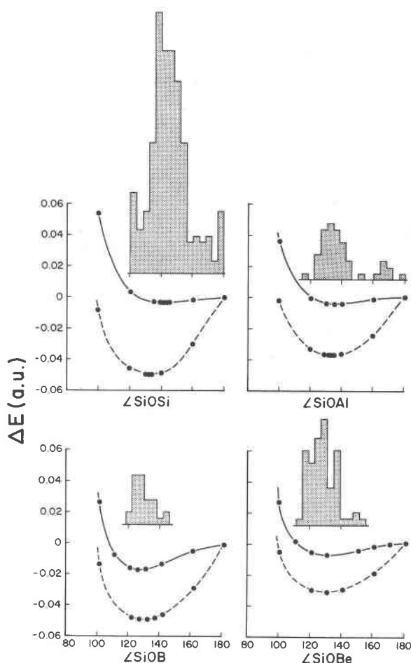
Fig. 13. Potential energy curves for the H_6SiTO_7 and H_7SiTO_7 molecules ( T = Si, Al, B, Be ) displayed as a function of (a) \angle SiOSi , (b) \angle SiOAl , (c) \angle SiOB and (d) \angle SiOBe (after Downs and Gibbs, 1981). Each curve was calculated using the optimized bridging bond lengths given in Table 2; the solid and dashed curves were calculated for H_6SiTO_7 and H_7SiTO_7 , respectively. The histogram superimposed above each pair of curves is a frequency distribution of the experimental SiOT bridging angles recorded for various silicates. (After Geisinger and Gibbs, 1981b.)
