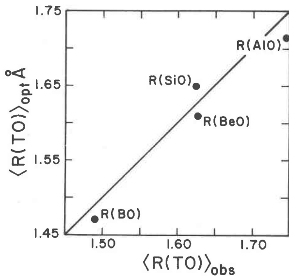
Fig. 14. The averaged tetrahedral bond lengths, \langle R(TO) \rangle_{opt.} , optimized for the molecules in Table 2 versus the averaged bridging bond lengths, \langle R(TO) \rangle_{obs.} , involving the angles used to prepare the histograms in Figure 13. The 45^\circ line represents the points of perfect agreement. (After Geisinger and Gibbs, 1981b.)
