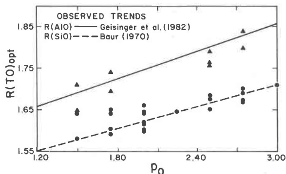
Fig. 16. Bridging tetrahedral TO ( T = \text{Al, Si} ) bond lengths, R(\text{TO})_{\text{opt}} , optimized for a number of molecules versus the bond strength sums, p_0 , of the bridging oxygen atoms. The R(\text{SiO}) and R(\text{AlO}) data are plotted as bullets and triangles, respectively. The lines drawn through the two trends were obtained in regression analyses of observed tetrahedral AlO and SiO bond length data versus p_0 for a large number of silicates. (After Geisinger and Gibbs, 1981b.)
