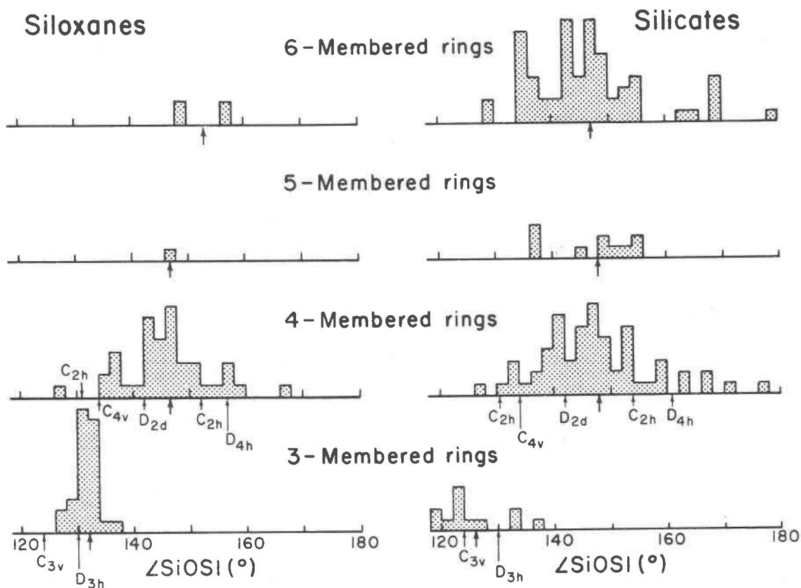
Fig. 9. The SiOSi angle frequency distributions for rings of disiloxy groups in silicates and siloxanes. The average angle for each distribution is represented by a boldface arrow while regular arrows mark the SiOSi angles of cyclotrisiloxane and cyclotetrasiloxane molecules optimized for various point symmetries. The point symmetries assumed in optimization of the angles are stated at the origin of each regular arrow. (After Chakoumakos, 1981.)
