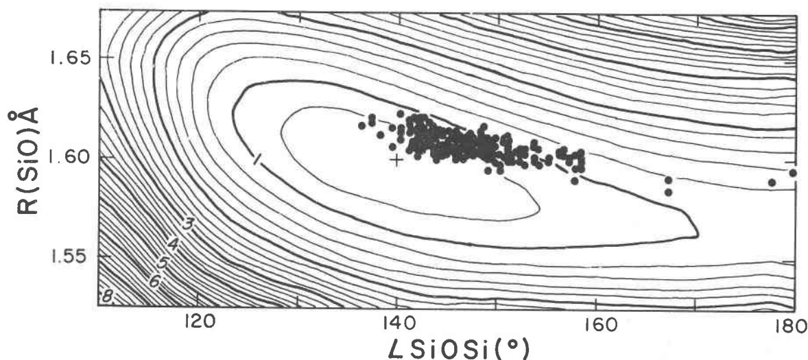
Fig. 8. A potential energy surface for the disilicate molecule, \text{H}_6\text{Si}_2\text{O}_7 , plotted as a function of its bridging bond length, R(\text{SiO}) , and \text{SiOSi} angle. The energy represented by the contours corresponds to increments of 0.001 a.u. ( = 0.6257 \text{ kcal mole}^{-1} ) relative to the minimum energy point ( -1091.76678 \text{ a.u.} ) denoted by a cross. For sake of convenience, the 0.005 a.u. increments are indicated by heavier lines labeled from 1 to 8 in order of increasing energy. The data points plotted on the energy surface are experimental bond lengths and angles for the disiloxo groups in the silica polymorphs coesite, tridymite, low cristobalite and \alpha -quartz. (After Meagher et al. , 1980.)
