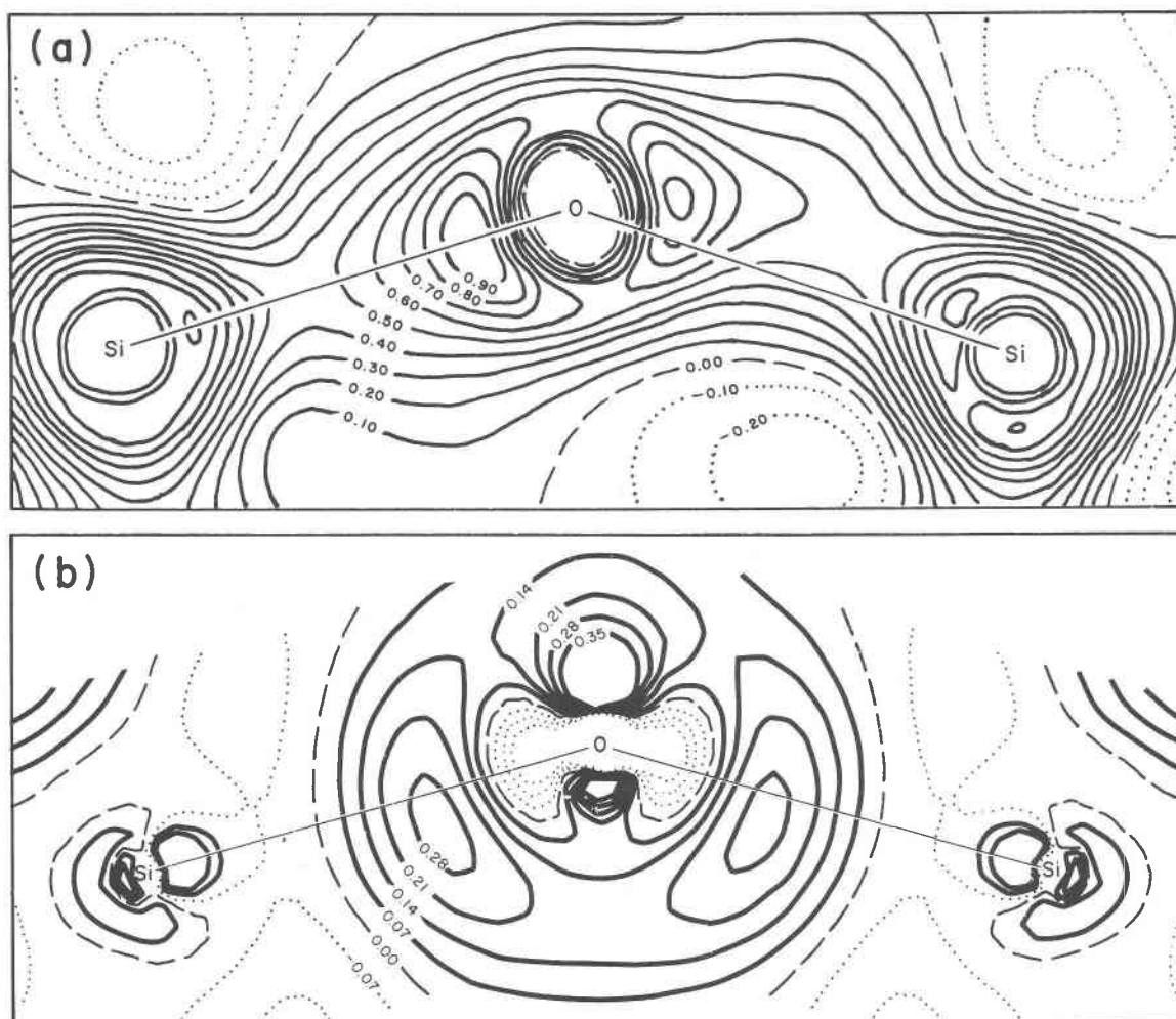
Fig. 11. Comparison of an experimental static deformation map (a) of the disiloxo group in \alpha -quartz with a theoretical map (after Spackman et al. , (1981) (b) of the bond in disiloxane calculated with a 66-31G* basis (after Gibbs and Newton, in prep.). The contours are drawn at intervals of 0.10 \text{ e } \text{\AA}^{-3} in (a) and 0.07 \text{ e } \text{\AA}^{-3} in (b).
