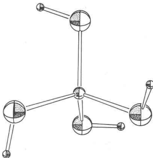
Fig. 1. A drawing of the molecular structure of monosilicic acid, \text{H}_4\text{SiO}_4 , as determined by molecular orbital methods. The intermediate-sized sphere at the center of the molecule represents a silicon atom, and the four large spheres disposed at the corners of a tetrahedron and attached to Si represent oxygen atoms. The small sphere attached to each oxygen atom represents hydrogen. No significance is attached to the relative sizes of the spheres. (After Gibbs et al. , 1981.)
