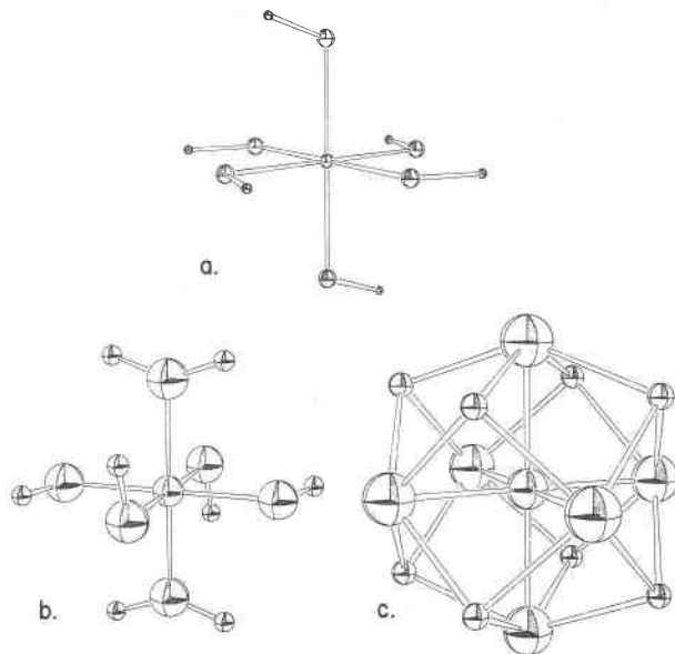
Fig. 4. Drawings of the molecules (a) \text{Si}(\text{OH})_6^{2-} , (b) \text{Si}(\text{OH})_4(\text{OH}_2)_2 and (c) \text{H}_8\text{SiO}_6 . The silicon atom centering each of these molecules is represented by an intermediate-size sphere, the six coordinating oxygen atoms disposed at the corners of a perfect octahedron are each represented by a large sphere, and the hydrogen atoms attached to the oxygen atoms are each represented by a small sphere. The point symmetries of \text{Si}(\text{OH})_6^{2-} and \text{Si}(\text{OH})_4(\text{OH}_2)_2 are both C_i whereas that of \text{H}_8\text{SiO}_6 is H_h . No significance is attached to the relative sizes of the spheres used to represent the atoms. (After Hill et al. , 1981.)
