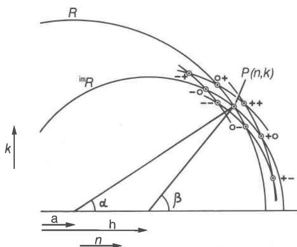
Fig. 3. The position of a point P(n, k) at the intersection of the true reflectance curves R and ^{im}R , and its angular position on the curves ( \alpha and \beta ). The intersection angle is the (acute) angle \beta - \alpha , and a and h are the distances of the centres of the true curves from the origin [see text, equation (3)]. A derived point P'(n', k') lies in the region bounded by arcs of curves for which the measured reflectances are in error; limiting points of this region are labelled (+o) and so on (i.e. R too high, ^{im}R no error, etc.).
