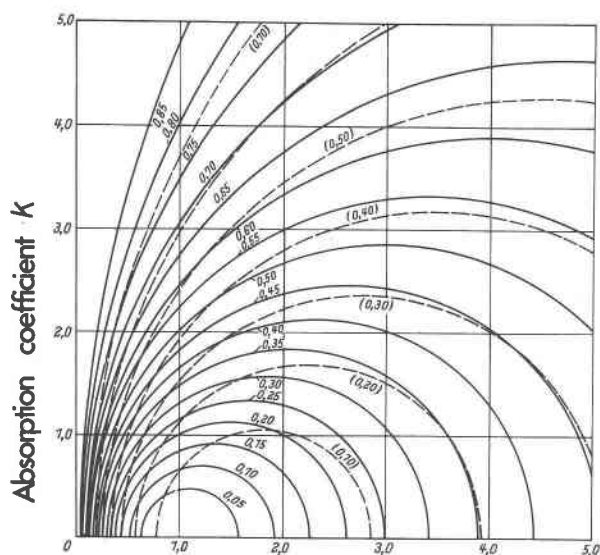
Fig. 1. The relations between the reflectance curves for air (solid) and oil (dashed) and the optical constants n and k (copied from Pepperhoff, 1965, p. 943, Fig. 1). See also Fig. 3. Reflectances are shown as decimal fractions, not as percentages.
