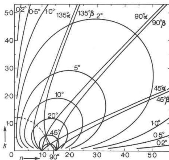
Fig. 2. Contours of constant intersection angle of the reflectance curves for air and oil ( N = 1.515 ), and of the angular positions of the intersection on the two curves, \alpha (air) and \beta (oil). The intersection contours should all meet at n = 1 and n = N . The dashed quarter-circle is the locus of intersections of curves for which R = {}^{\text{im}}R ; the equation is n^2 + k^2 = N . The locus of intersections of curves of equal radius lies between the curves \alpha = 90^\circ and \beta = 90^\circ , but is not shown.
