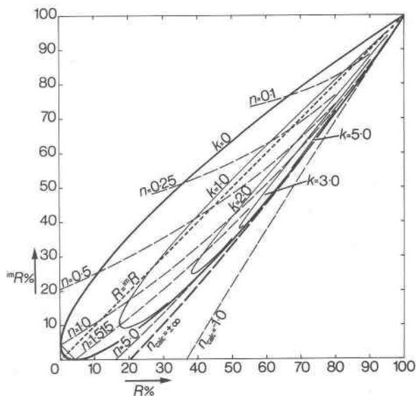
Fig. 4. The R/^{im}R cigar diagram (drawn for N = 1.515 ). The field of real values of n and k (absorption coefficient) lies inside the k = 0 contour. Above the cigar, and between it and the curve n(\text{calc}) = \pm\infty , k(\text{calc}) is complex and n(\text{calc}) real but false; below the curve n(\text{calc}) = \pm\infty , k(\text{calc}) is complex and n(\text{calc}) negative. The short line joining the points where the cigar touches the axes (bottom left) is the 90^\circ intersection contour, the only one shown; the small region of obtuse intersections lies between it and the origin inside the cigar, and contours of acute intersections lie in the remainder of the cigar. The locus of intersections between reflectance curves of equal radius (not drawn) joins the 'blunt ends' of the k contours; the curves \alpha = 90^\circ and \beta = 90^\circ lie on either side of it (cf. Fig. 2).
