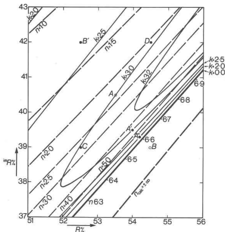
Fig. 5. An enlarged portion of the R/1mR cigar diagram ( N = 1.515 ). The points A and B represent measured values for pyrite, and A is assumed to be near the true value. B' , C , and D are points with the same size errors as B , but of different sign combinations; A' and A'' lie between A and B , with smaller errors than B (see text). Intersections of n contours with k = 0 are indicated by the value of n .
