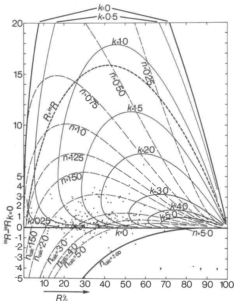
Fig. 6. Variant of the cigar diagram (drawn for N = 1.515 ). The lower part of the k = 0 curve is the horizontal straight line from the origin, and the locus of R = 100R_k=0 is the dashed curve (cf. Fig. 4). Horizontal units are in R percent; vertical units in 100R percent above the k = 0 boundary, i.e. 100R_{n,k} - 100R_{k=0} , and all points below k = 0 are in the imaginary field. All k contours are terminated 0.1 percent above the k = 0 datum. The plotted points are for 194 pairs of air and oil reflectances at 589 nm, and are taken from the IMA/COM Data File 1977.
