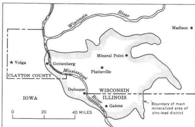
FIG. 1. Location of Volga, Iowa, and boundary of the main mineralized area of the Upper Mississippi Valley zinc-lead district.
