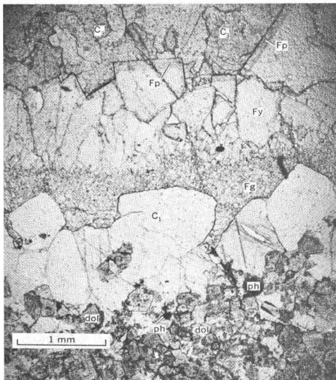
FIG. 9. Photomicrograph of crustified minerals on phosphatic dolomite of wallrock. Stages 1 and 3 calcite ( C_1 , C_3 ); colorless granular, yellow, and purple fluorite (Fg, Fy, Fp); dolomite (dol); phosphatic pellet (ph). Ordinary light.
