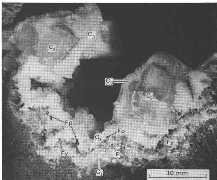
FIG. 6. Drusy vug showing overgrowth of stage 3 calcite and paragenetic relations of other minerals. Calcite stages ( C_1 , C_2 , C_3 ); pyrite (P); yellow and purple fluorite (Fy, Fp).
