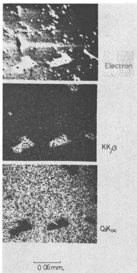
FIG. 3. The back-scattered electron and the \text{KK}\beta and \text{CaK}\alpha x-ray fluorescence photographs of the same small portion of an antiperthite crystal. The white areas marked 1 and 2 on the back-scattered electron photograph are the alkali feldspar aggregates studied in detail.
